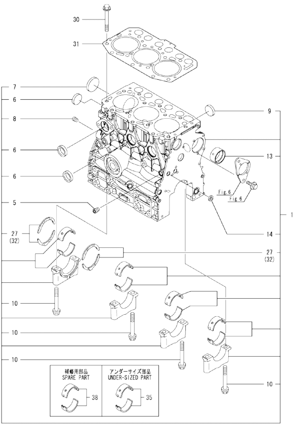
Fig.1. CYLINDER BLOCK
