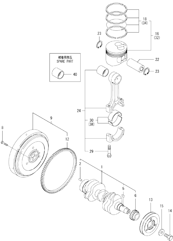
Fig.7. CRANKSHAFT & PISTON
