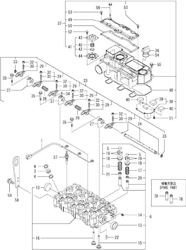
OCD10-M91301 3TNV70-XHB/3TNV70-XHBT Fig.4. CYLINDER HEAD & BONNET
