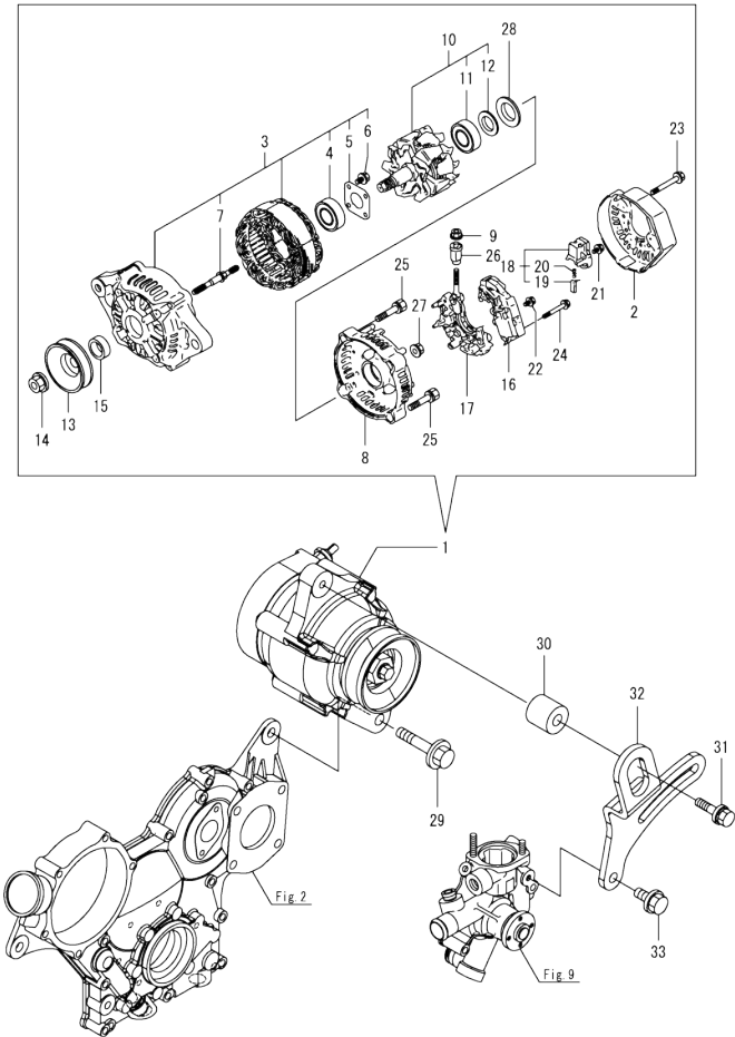
Fig.13. GENERATOR
