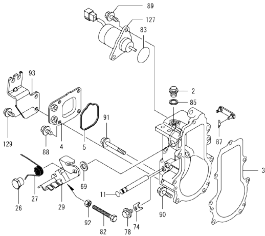
OCD50-M06030 ENGINE Fig.11. GOVERNOR
