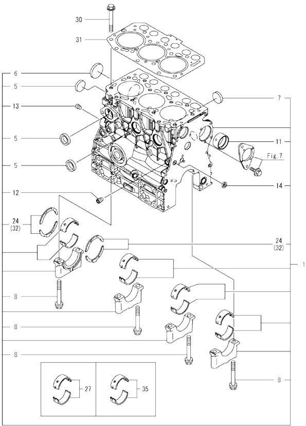
Fig.1. CYLINDER BLOCK
