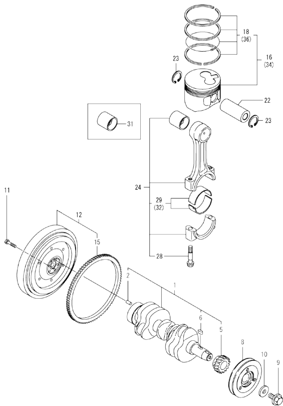
Fig.8. CRANKSHAFT & PISTON
