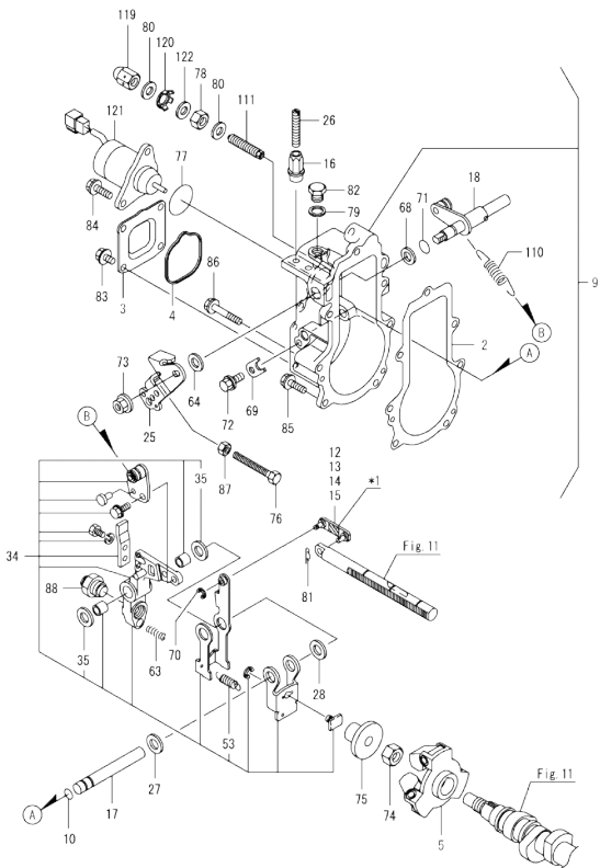
Fig.12. GOVERNOR
