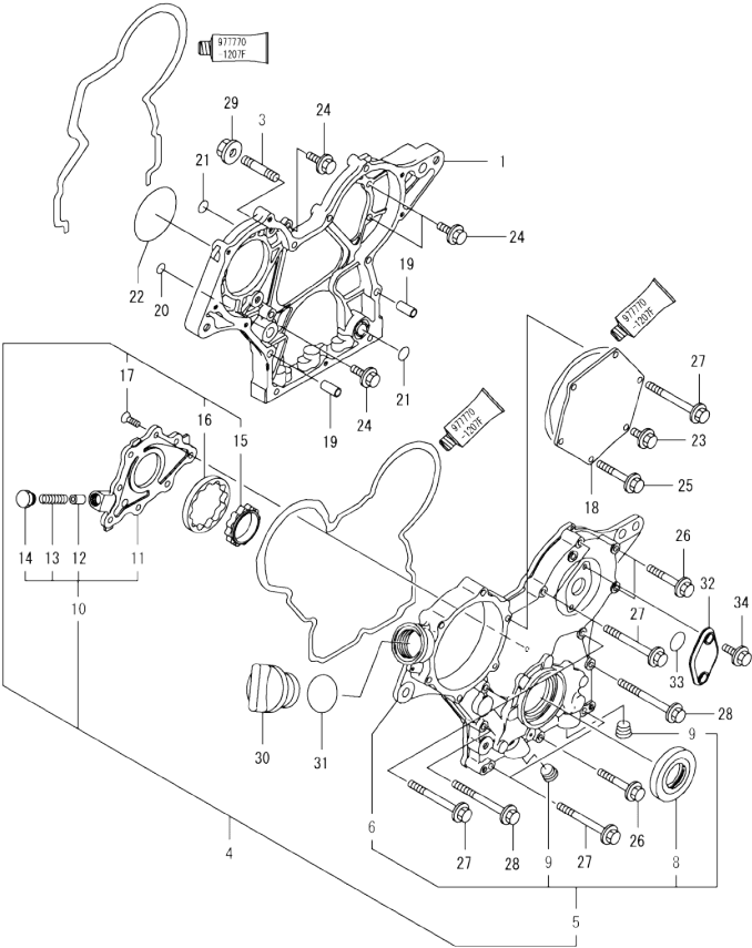
0CW10-M85500 3TNV70-XPLW Fig.2. GEAR HOUSING
