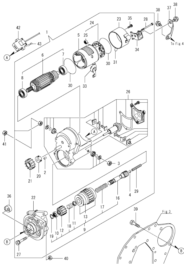
OCD50-M07130 ENGINE Fig.14. STARTING MOTOR
