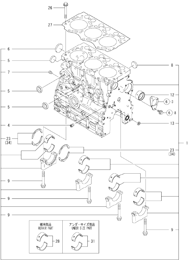
Fig.1. CYLINDER BLOCK
