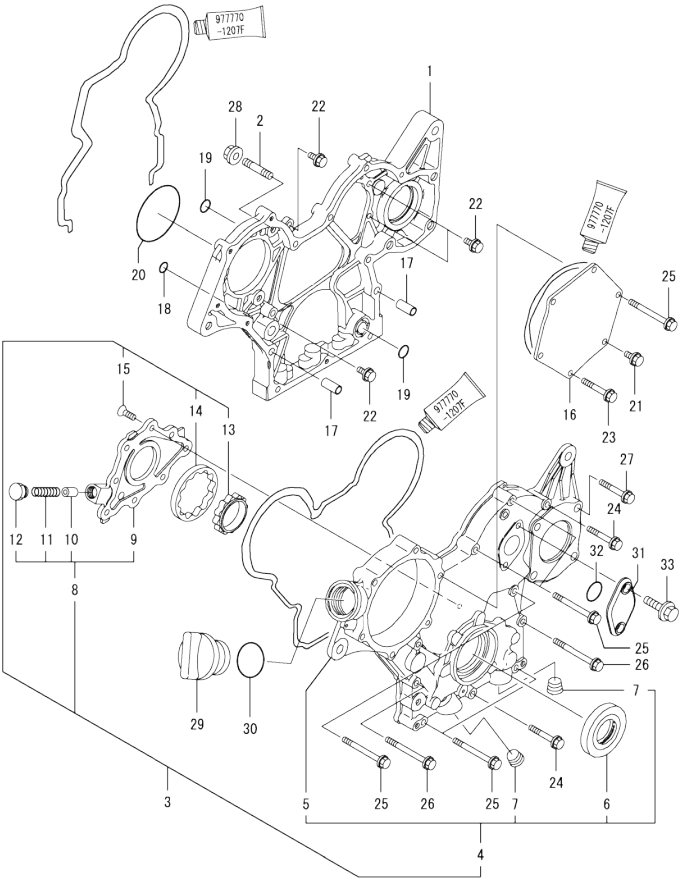
Fig.2. GEAR HOUSING
