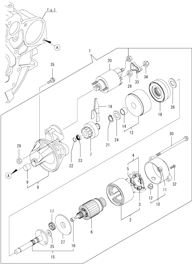
Fig.15. STARTER MOTOR
