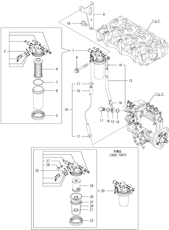
Fig.14. FUEL PIPE
