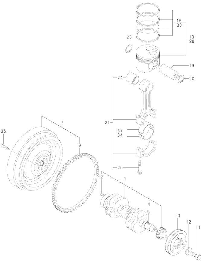
Fig.7. CRANKSHAFT & PISTON
