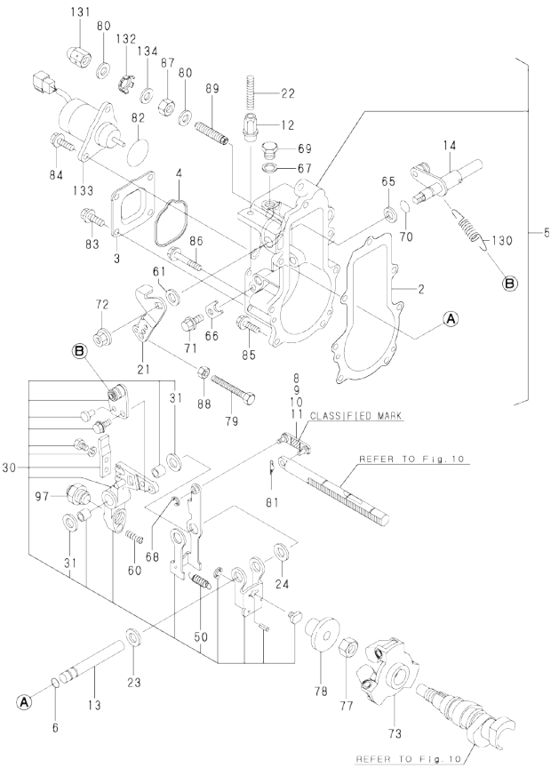
Fig.11. GOVERNOR
