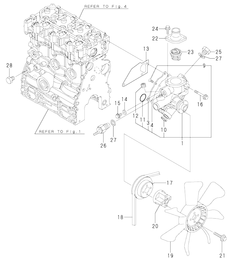
OCR10-M58100 ENGINE SECTION (3TNV76-CSA) Fig.9. COOLING WATER SYSTEM
