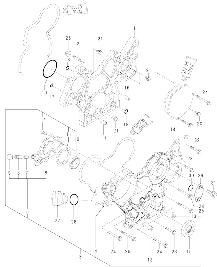
Fig.2. GEAR HOUSING
