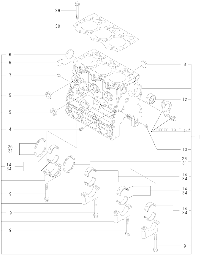
Fig.1. CYLINDER BLOCK
