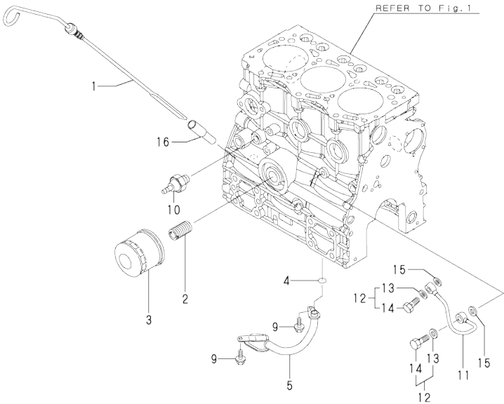
Fig.8. LUB.OIL SYSTEM
