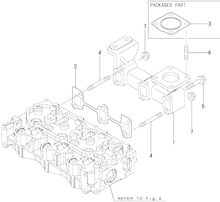
Fig.5. EXHAUST MANIFOLD
