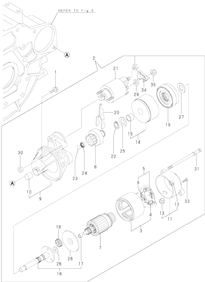
Fig.14. STARTING MOTOR
