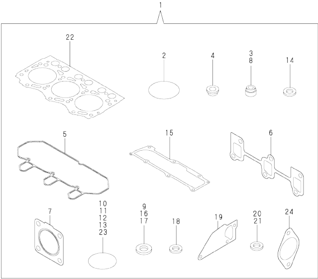
Fig.16. GASKET SET & TOOLS
