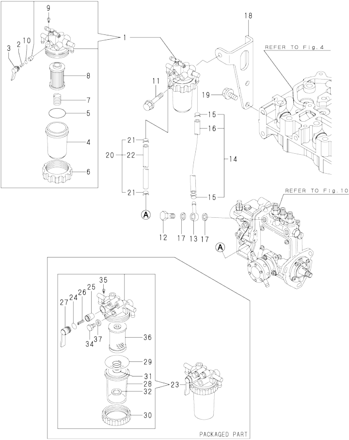
Fig.13. FUEL PIPE
