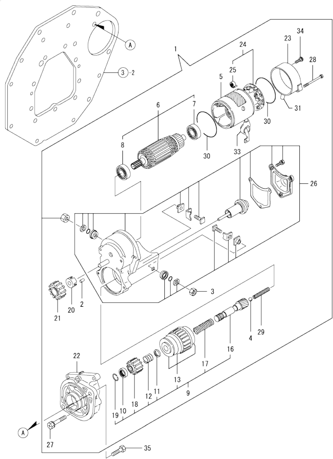
Fig.14. STARTING MOTOR
