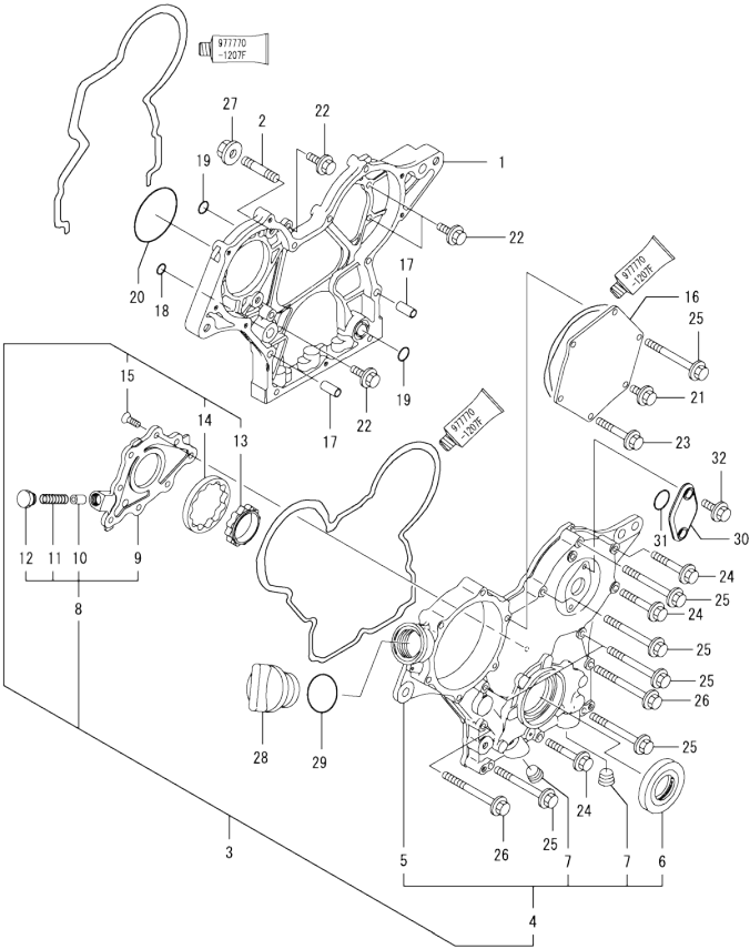
0CW10-M40800 3TNV76-DST Fig.2. GEAR HOUSING
