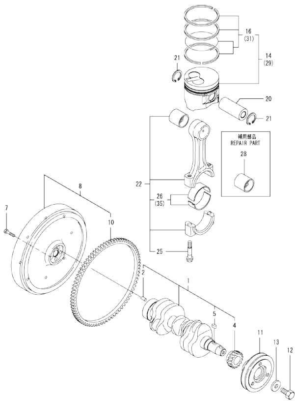
0CW10-M40800 3TNV76-DST Fig.8. CRANKSHAFT & PISTON
