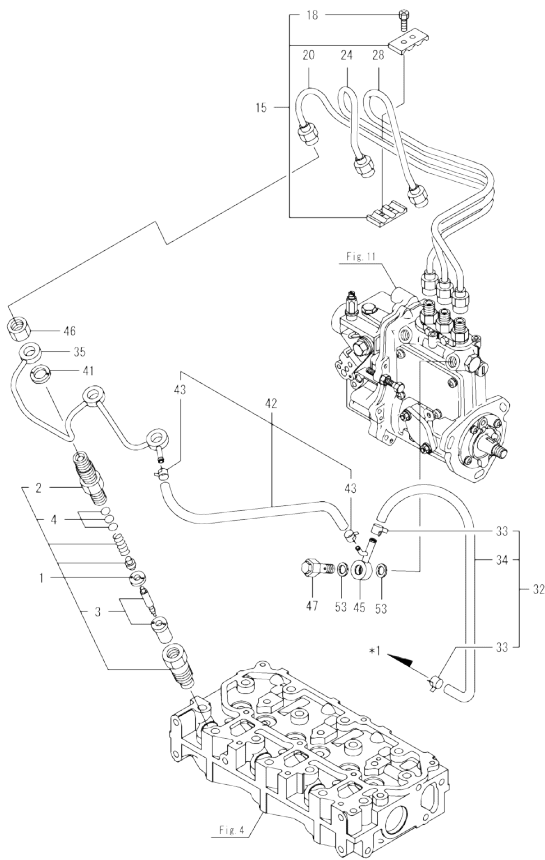
Fig.13. FUEL INJECTION VALVE
