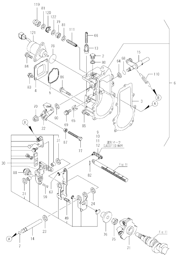
Fig.12. GOVERNOR
