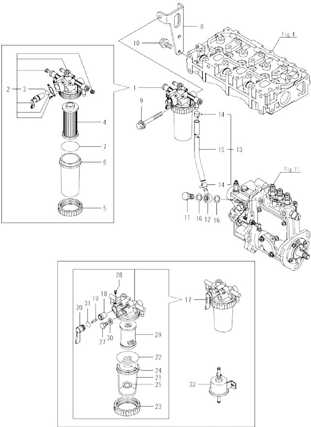
Fig.14. FUEL FILTER
