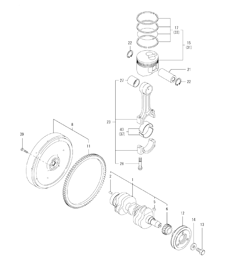
Fig.7. CRANKSHAFT & PISTON
