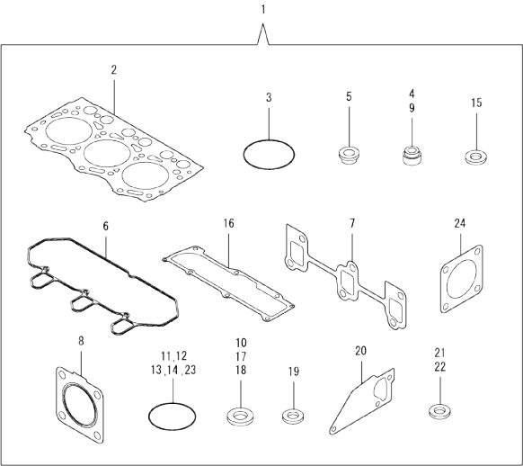
Fig.17. GASKET SET
