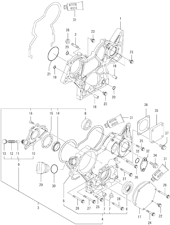
Fig.2. GEAR HOUSING
