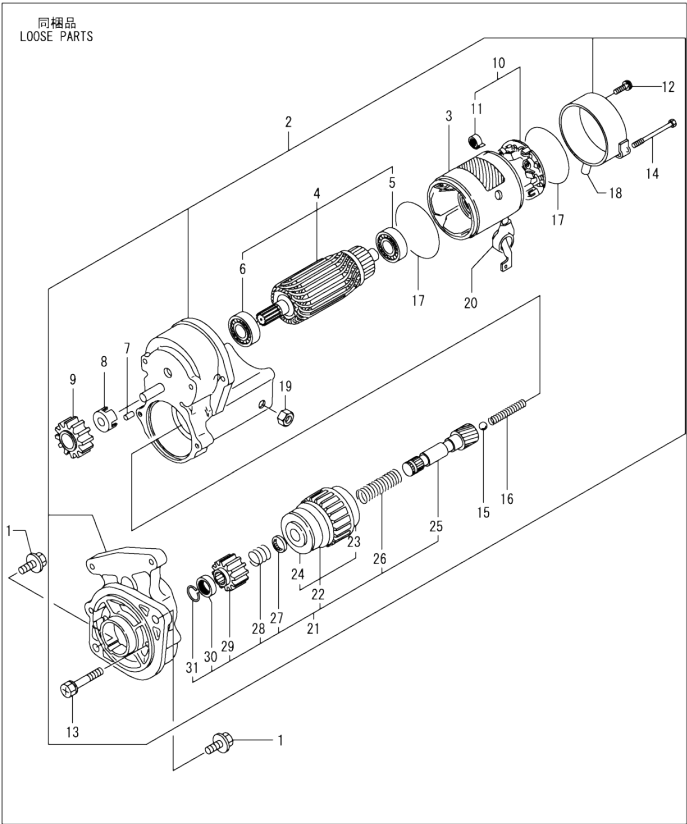
Fig.14. STARTING MOTOR
