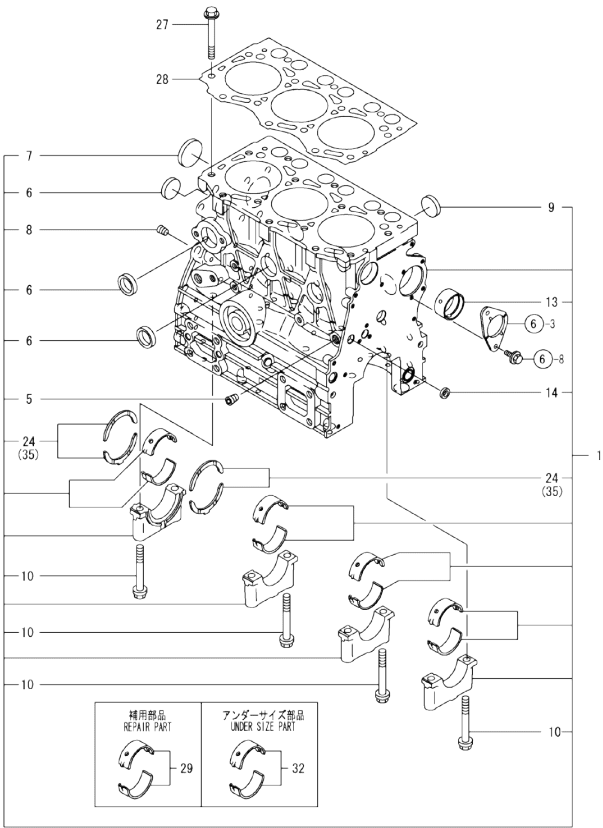
Fig.1. BLOCK, CYLINDER
