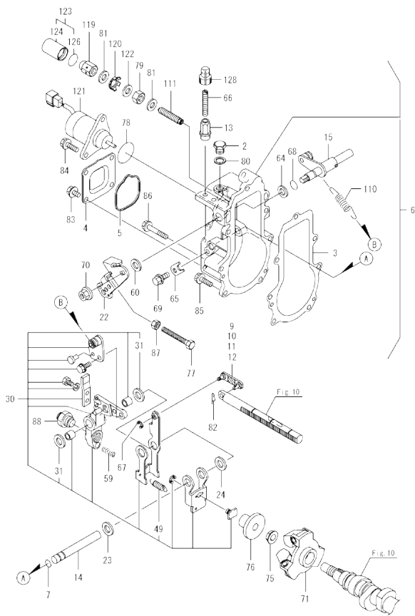
Fig.11. GOVERNOR
