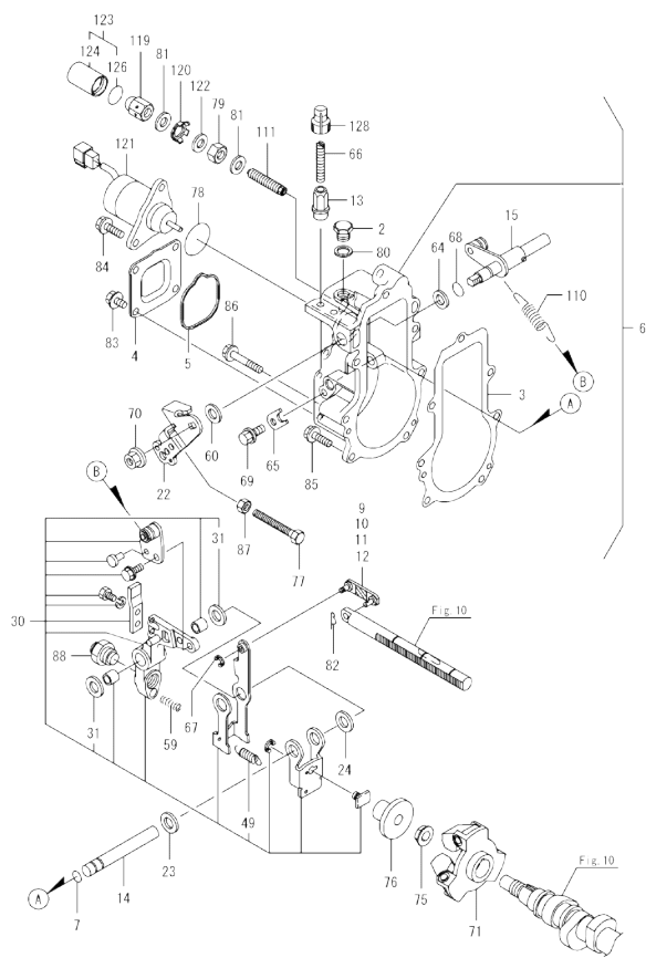
Fig.11. GOVERNOR
