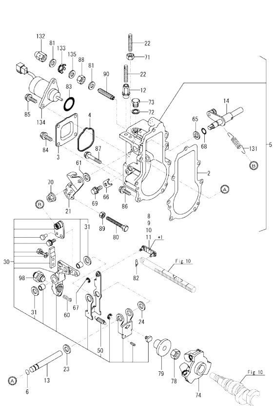
OCD10-M85201 ENGINE SECTION Fig.11. GOVERNOR
