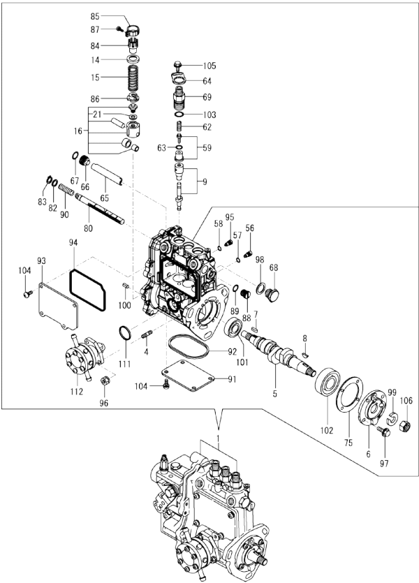
Fig.18. (10A)FUEL INJECTION PUMP
