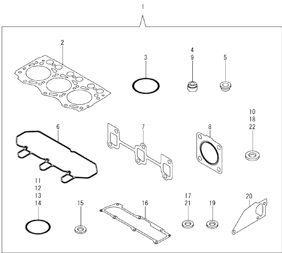
OCD10-M85201 ENGINE SECTION Fig.16. GASKET SET
