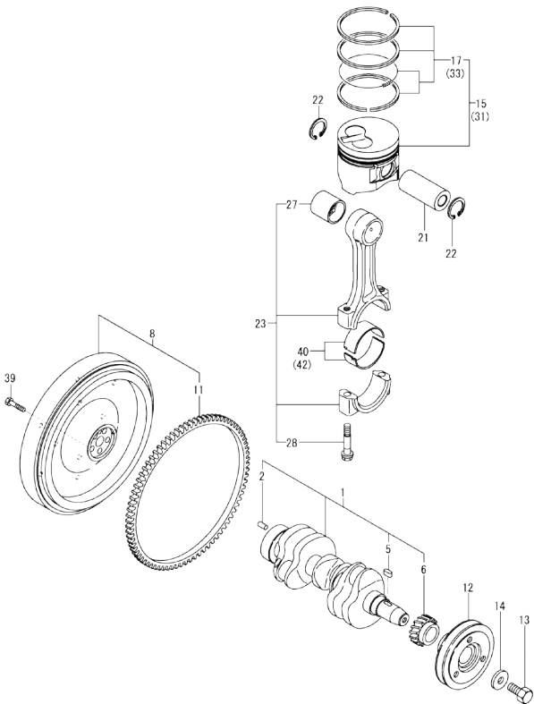
OCD10-M85201 ENGINE SECTION Fig.7. CRANKSHAFT & PISTON
