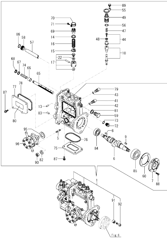
OCD10-M85201 ENGINE SECTION Fig.10. FUEL INJECTION PUMP
