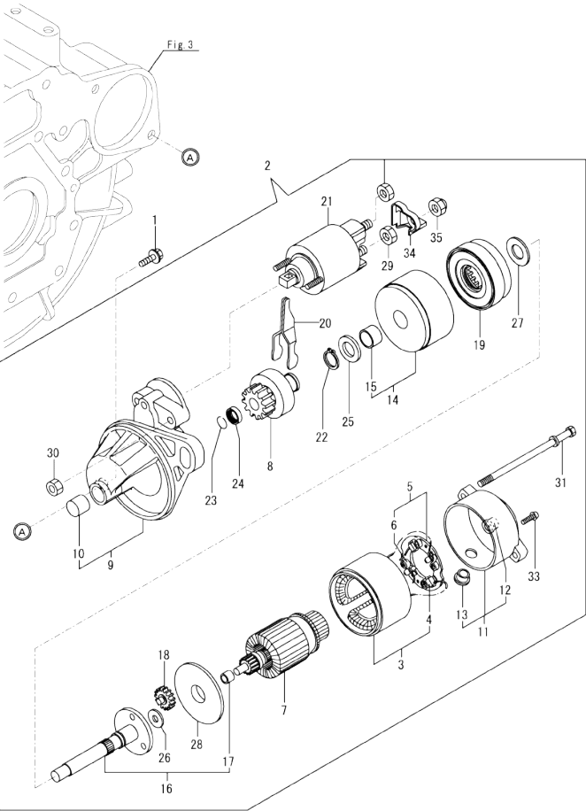
OCD10-M85201 ENGINE SECTION Fig.13. STARTER MOTOR
