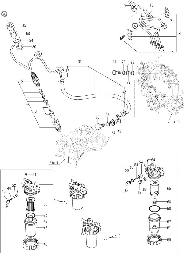
Fig.20. (12B)FUEL INJECTION VALVE
