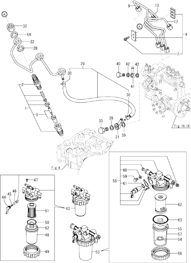
Fig.17. (12A)FUEL INJECTION VALVE
