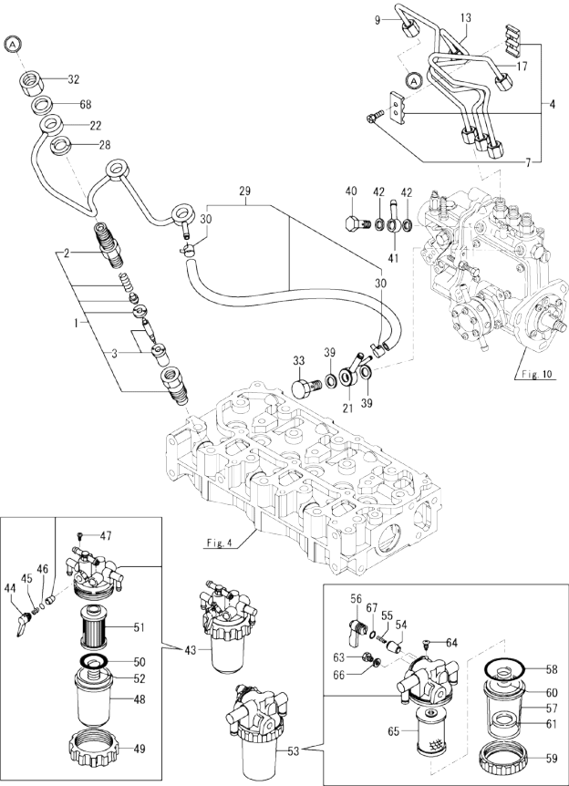
OCD10-M85201 ENGINE SECTION Fig.12. FUEL INJECTION VALVE
