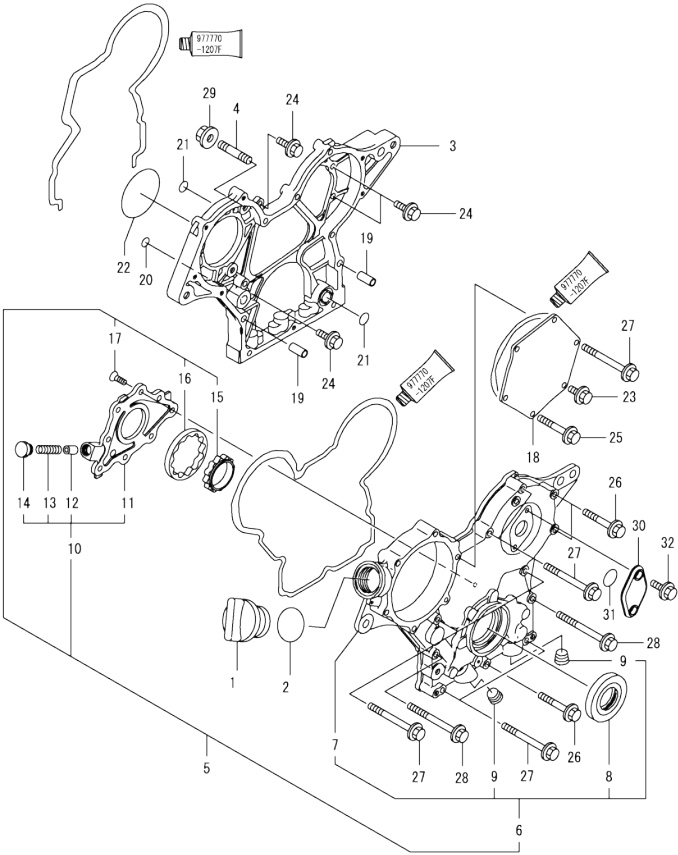
Fig.2. CASE, GEAR
