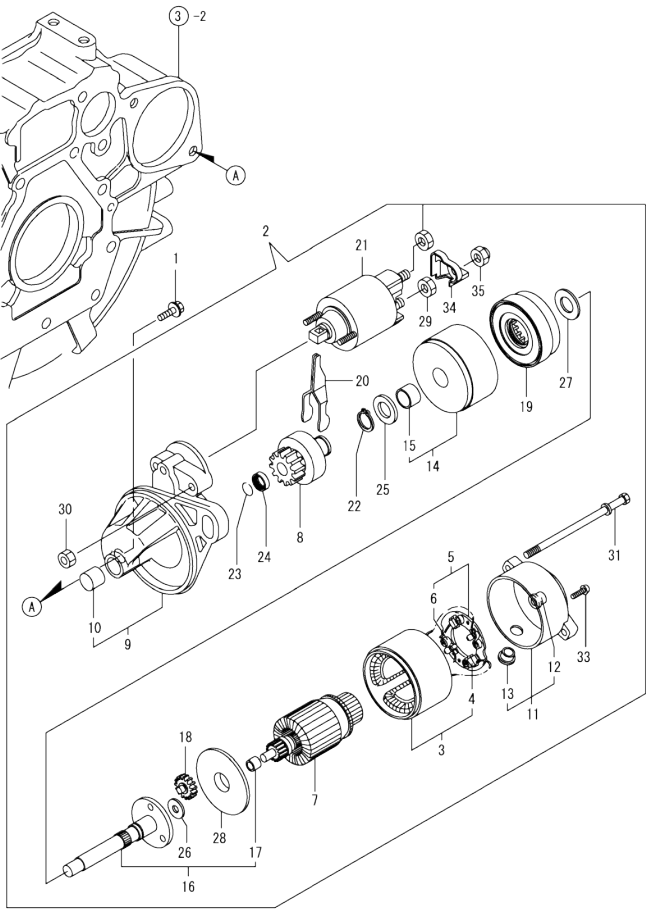
Fig.13. STARTING MOTOR
