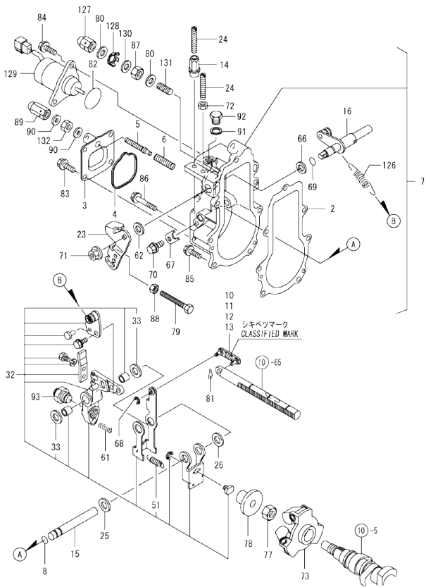
Fig.11. GOVERNOR
