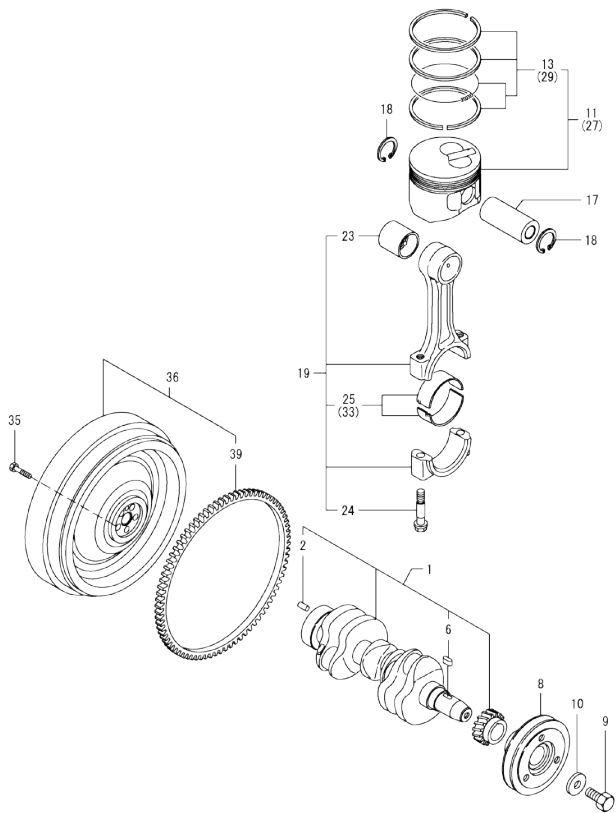
0CW10-M42100 3TNV76-GEU Fig.7. CRANKSHAFT & PISTON
