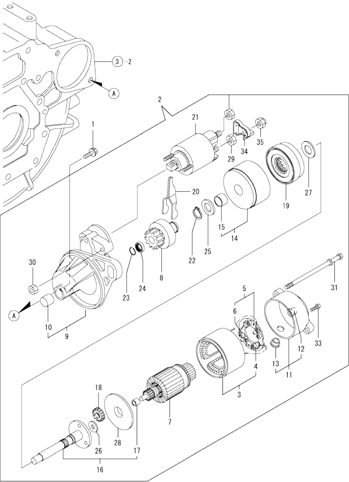
Fig.17. STARTER MOTOR
