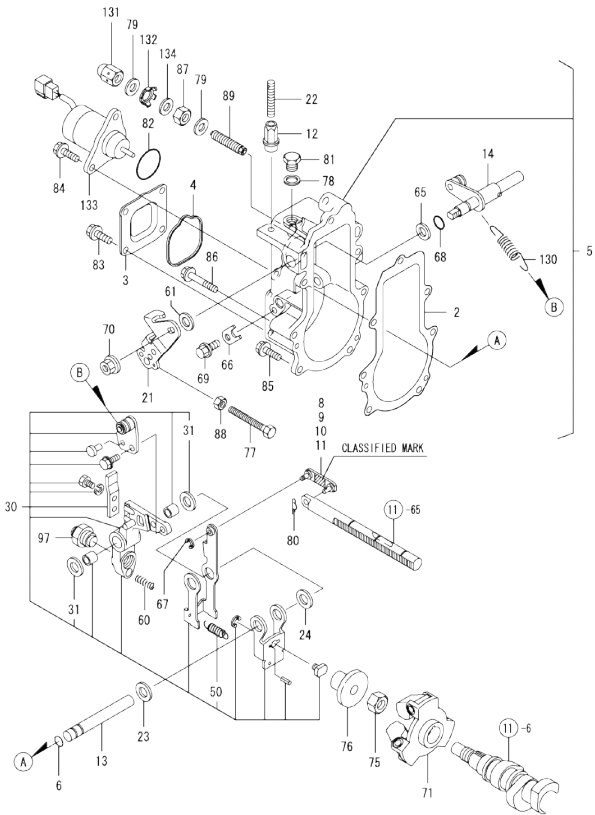
OCR10-M57400 ENGINE Fig.12. GOVERNOR
