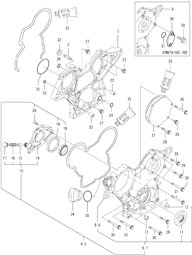
Fig.2. GEAR HOUSING
