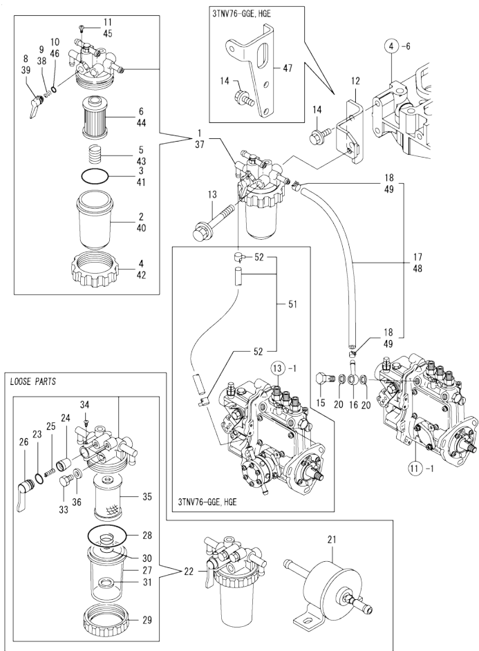
Fig.16. FUEL PIPING
