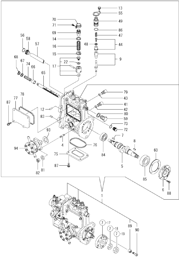
0CW10-M15900 3TNV76-GGEH Fig.11. FUEL INJECTION PUMP
