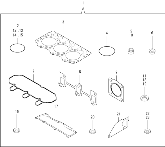
0CW10-M15900 3TNV76-GGEH Fig.17. GASKET SET
