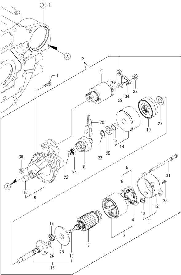
0CW10-M15900 3TNV76-GGEH Fig.15. STARTING MOTOR
