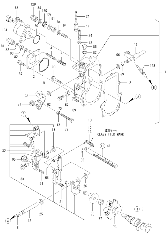
Fig.12. GOVERNOR
