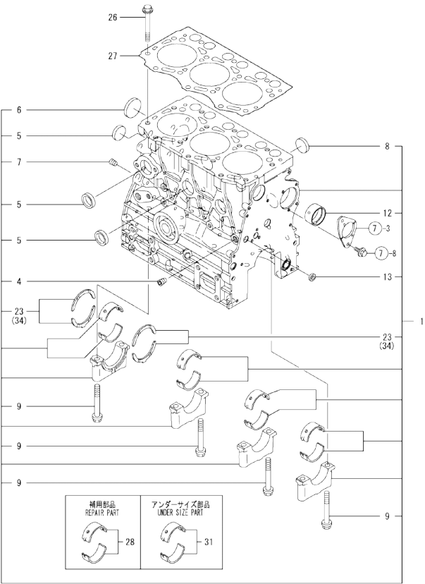
0CW10-M19400 3TNV76-GGEHC Fig.1. CYLINDER BLOCK
