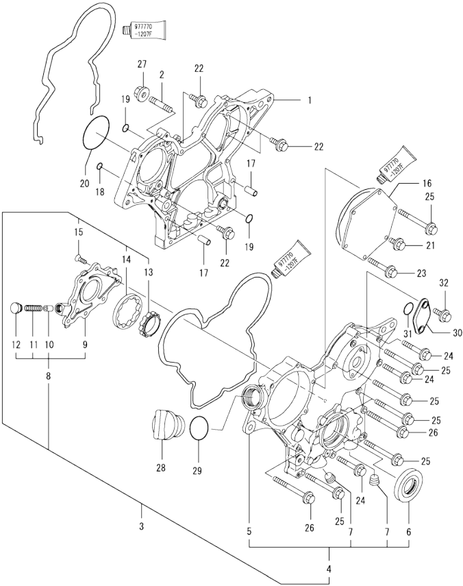
0CW10-M49600 3TNV76-GGK2 Fig.2. GEAR HOUSING
