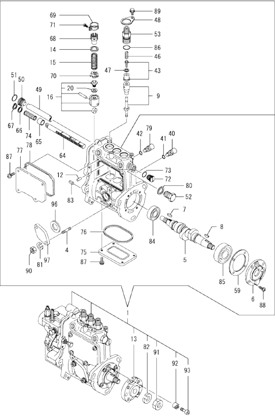
Fig.9. FUEL INJECTION PUMP
