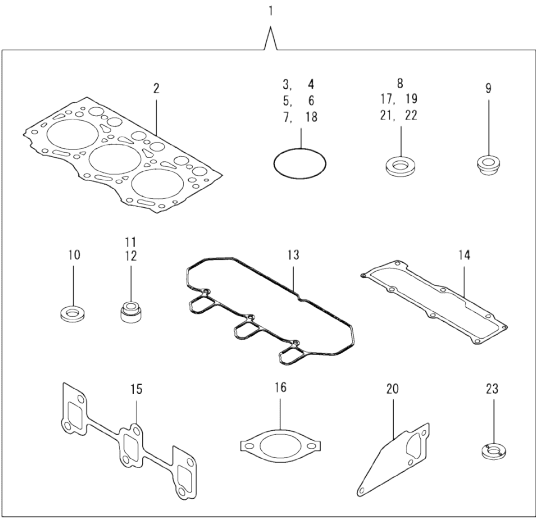
Fig.14. GASKET SET
