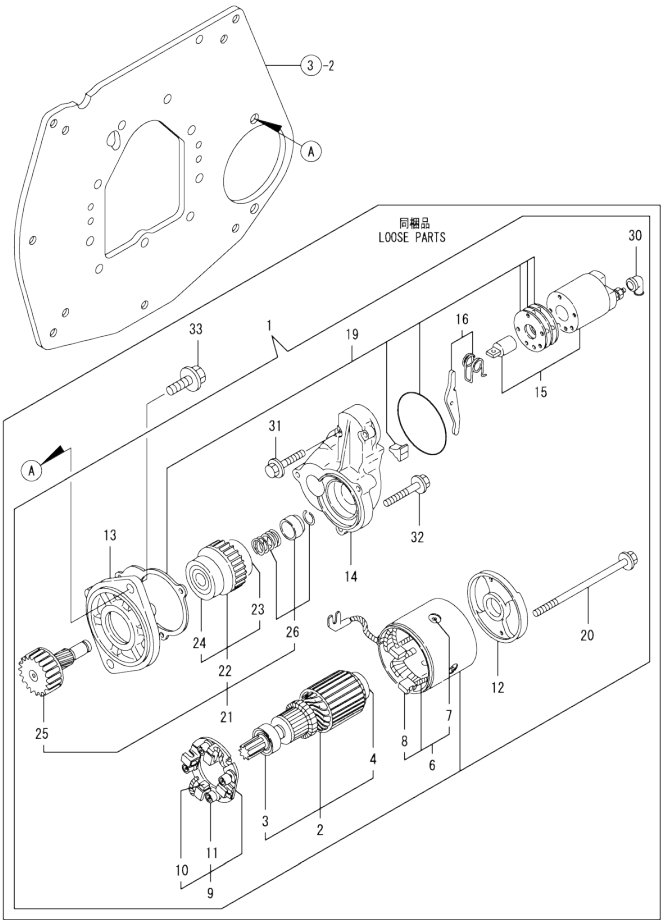
0CW10-M49600 3TNV76-GGK2 Fig.13. STARTING MOTOR
