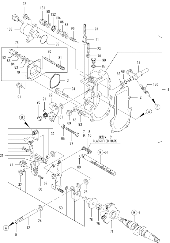
Fig.10. GOVERNOR
