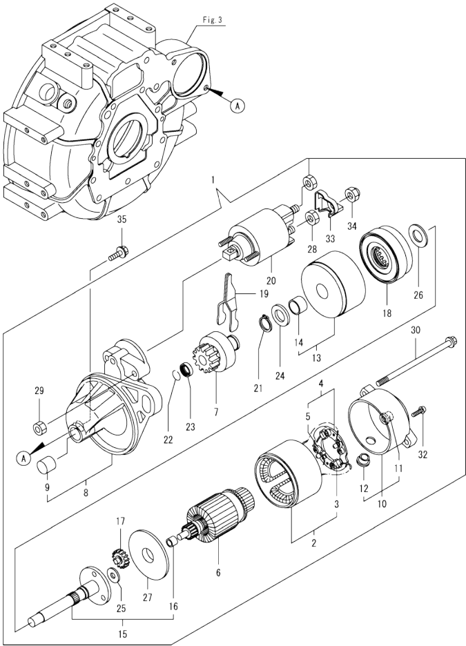
Fig.14. STARTER MOTOR
