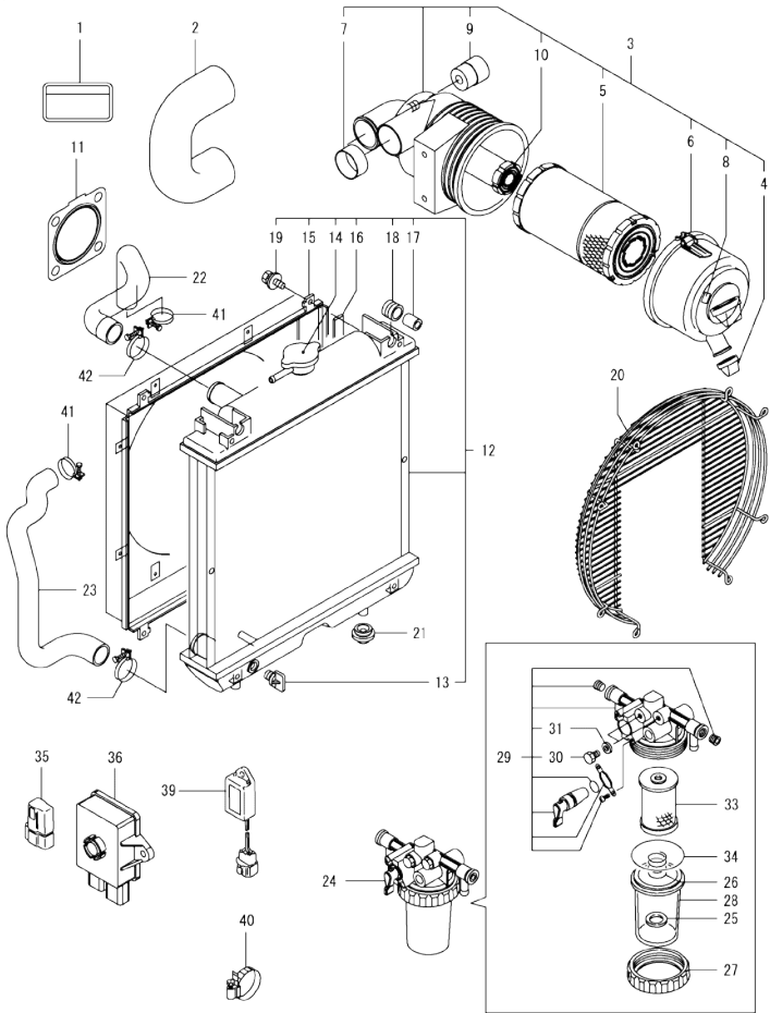
Fig.16. ACCESSORY
