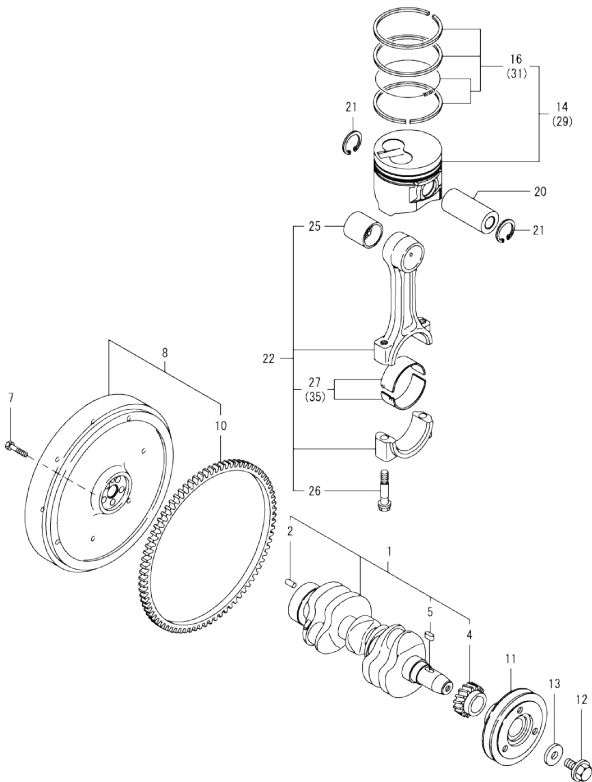
Fig.7. CRANKSHAFT & PISTON
