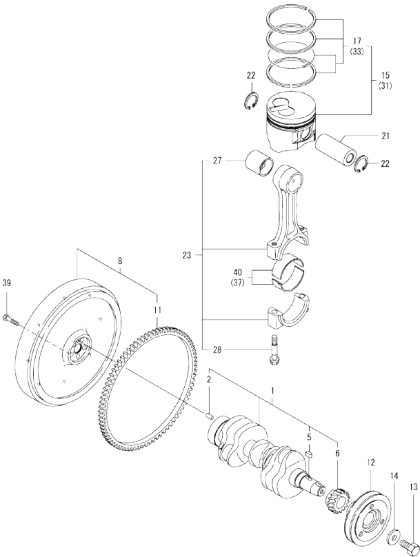
Fig.6. CRANKSHAFT & PISTON
