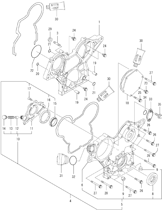
Fig.2. GEAR HOUSING
