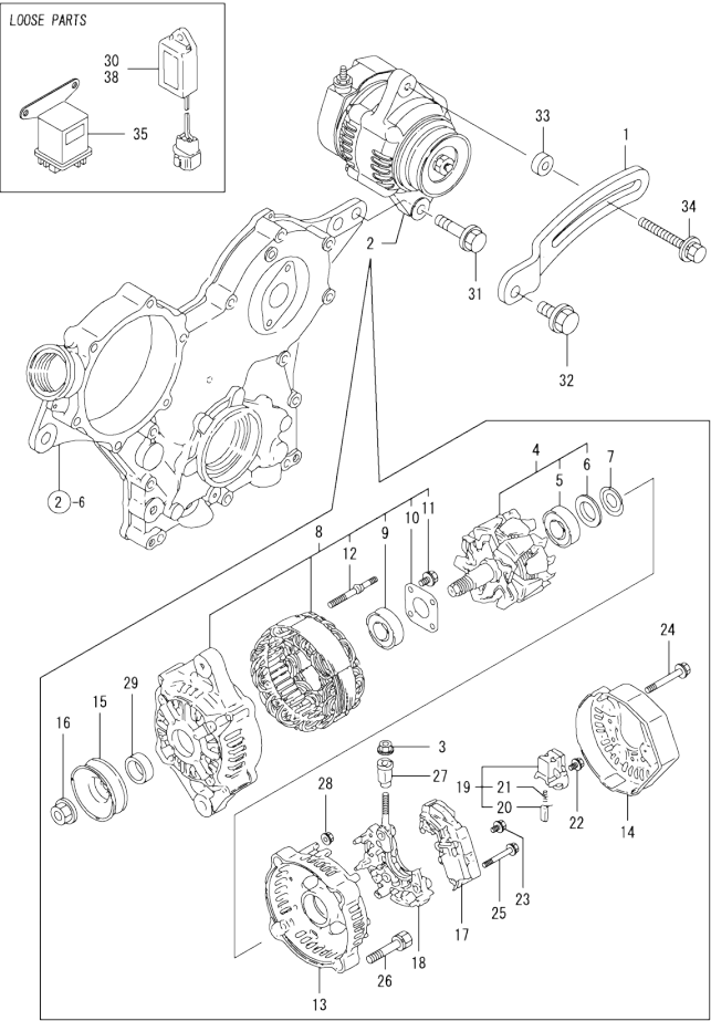
Fig.13. GENERATOR
