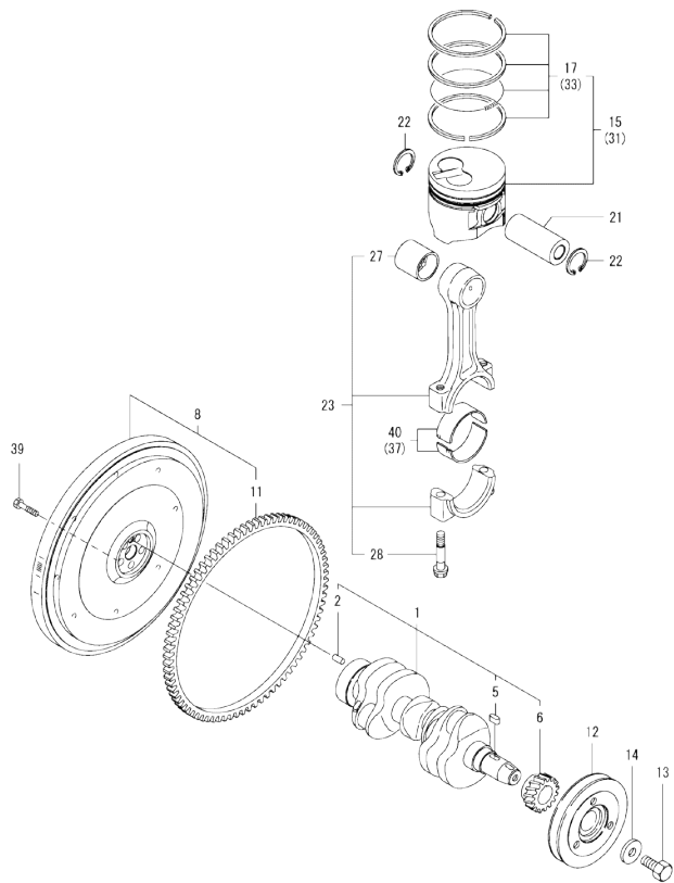
Fig.6. CRANKSHAFT & PISTON
