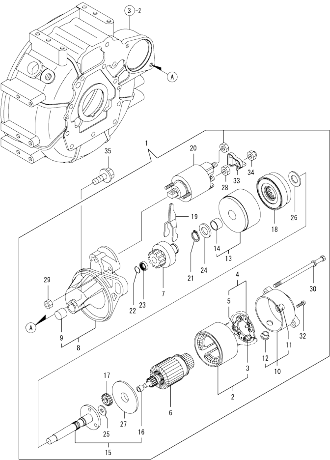
Fig.15. STARTING MOTOR
