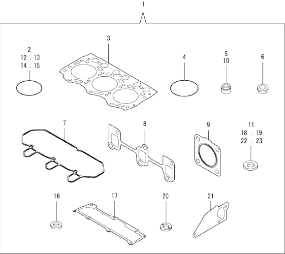
Fig.17. GASKET SET
