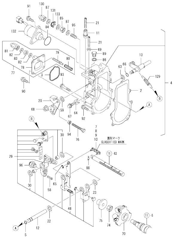
Fig.12. GOVERNOR
