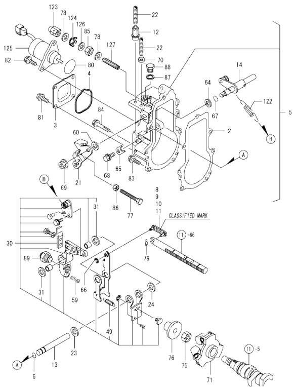
Fig.12. GOVERNOR
