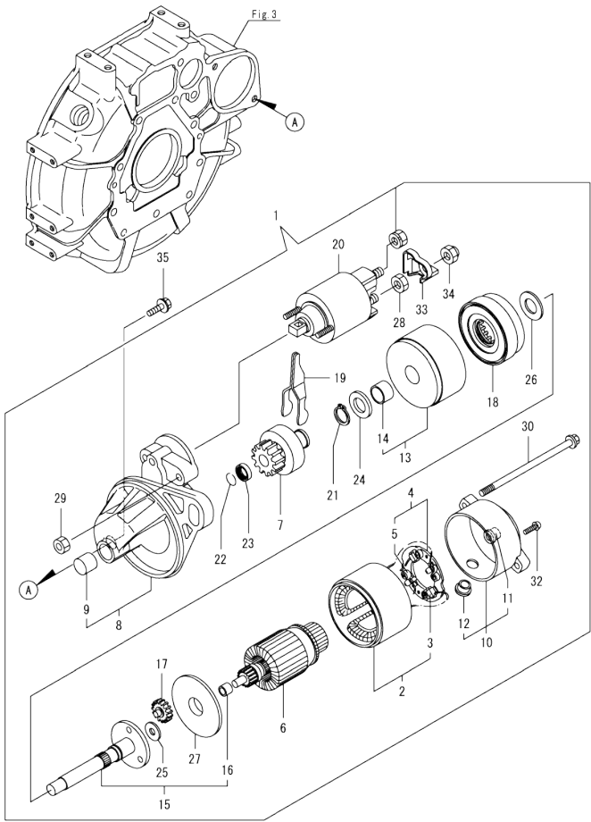
Fig.13. STARTER MOTOR
