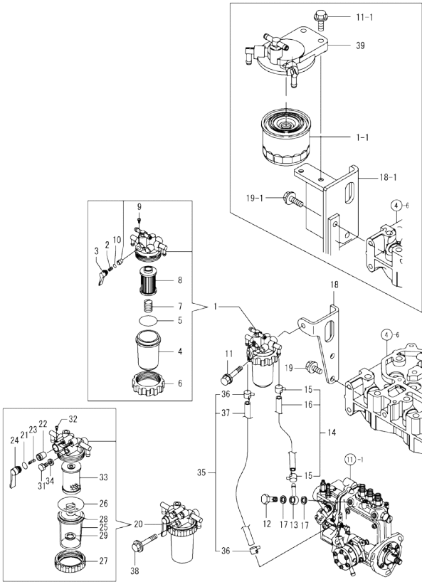
Fig.14. FUEL LINE
