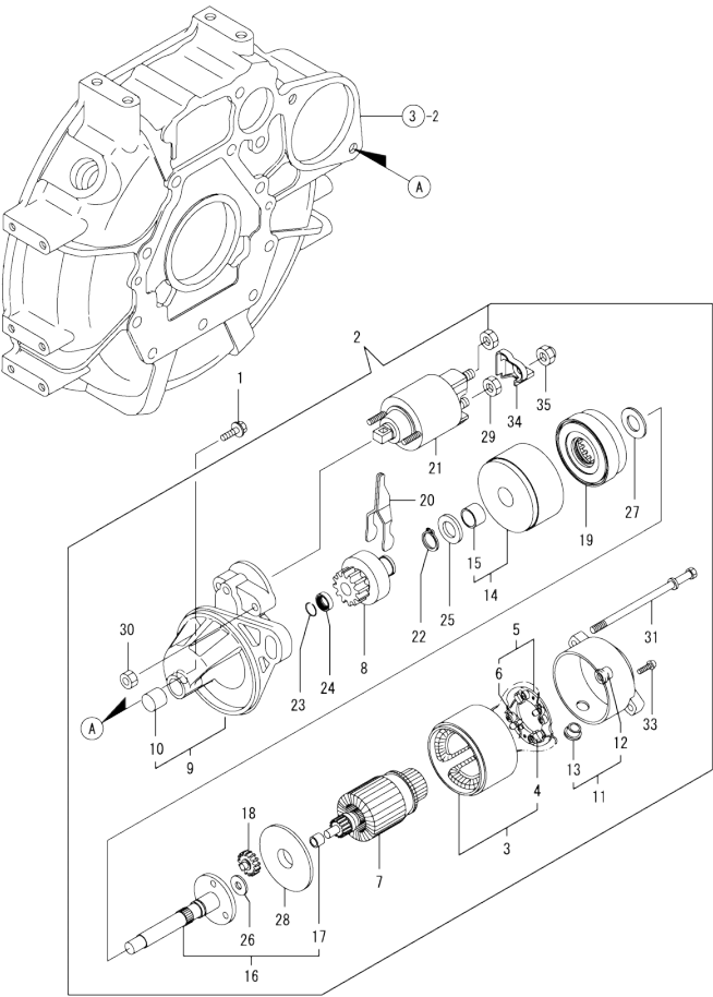
OCD10-M91700 ENGINE SECTION Fig.15. STARTING MOTOR
