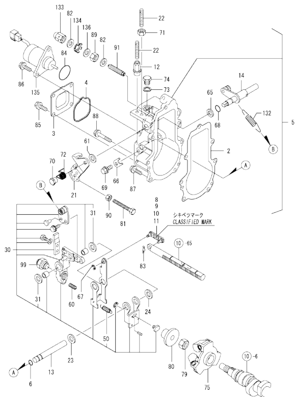
Fig.12. GOVERNOR
