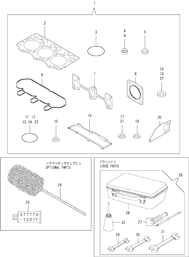
OCD10-M91700 ENGINE SECTION Fig.17. GASKET SET & TOOLS
