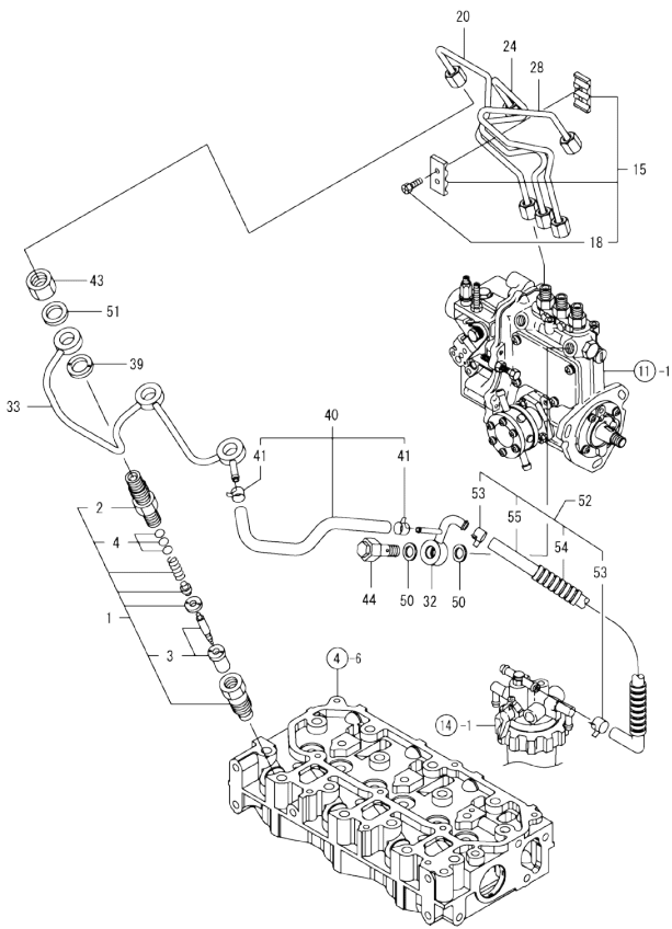
OCD10-M91700 ENGINE SECTION Fig.13. FUEL INJECTION VALVE
