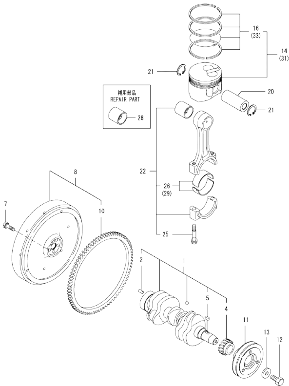
Fig.8. CRANKSHAFT & PISTON
