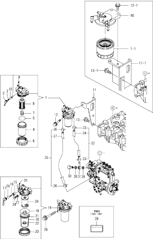
Fig.14. FUEL LINE
