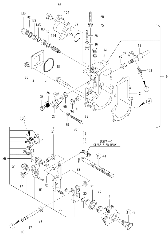
Fig.12. GOVERNOR
