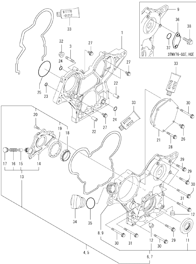
Fig.2. GEAR HOUSING
