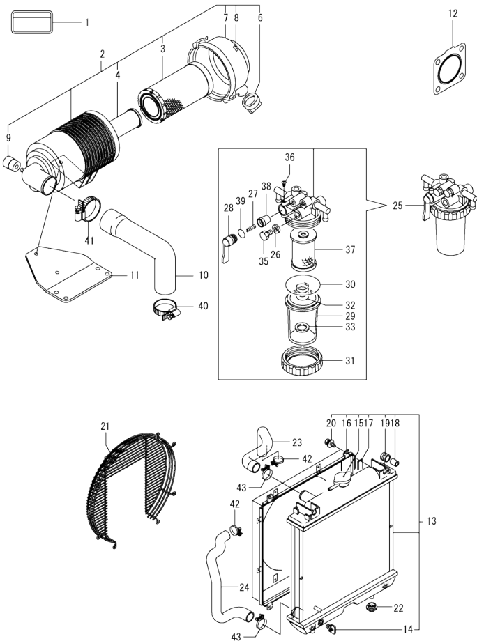
Fig.16. ACCESSORY
