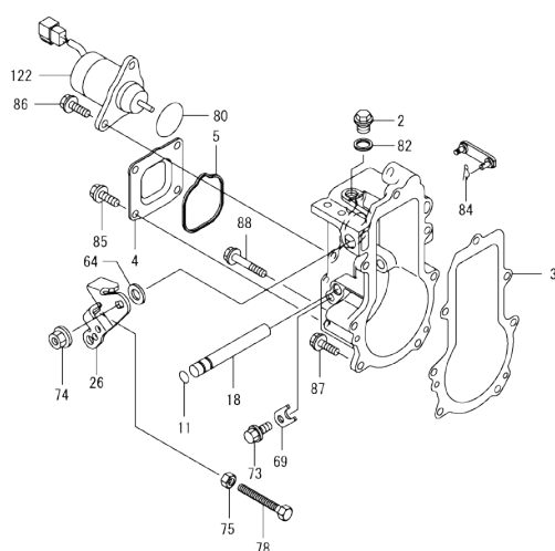
Fig.11. GOVERNOR
