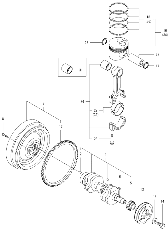
Fig.7. CRANKSHAFT & PISTON
