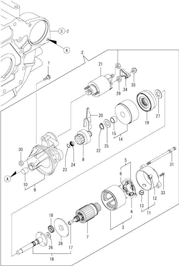
Fig.17. STARTING MOTOR
