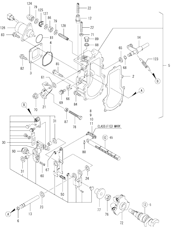
Fig.13. GOVERNOR
