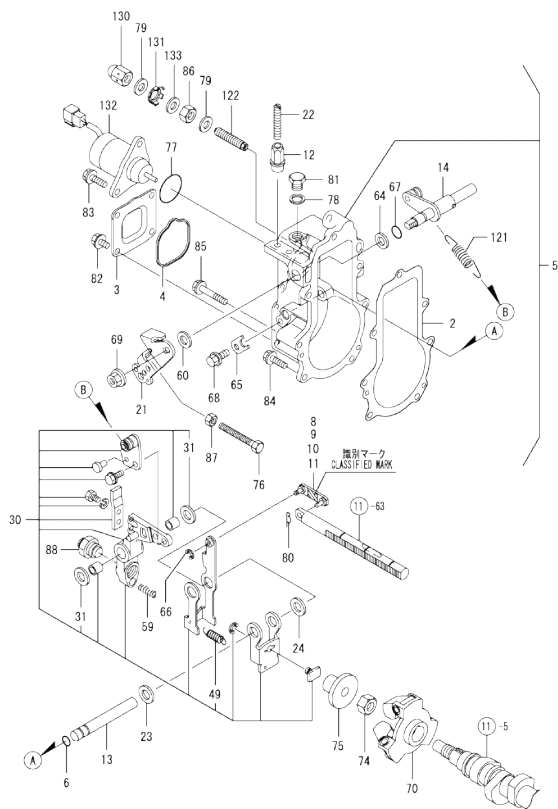
Fig.12. GOVERNOR
