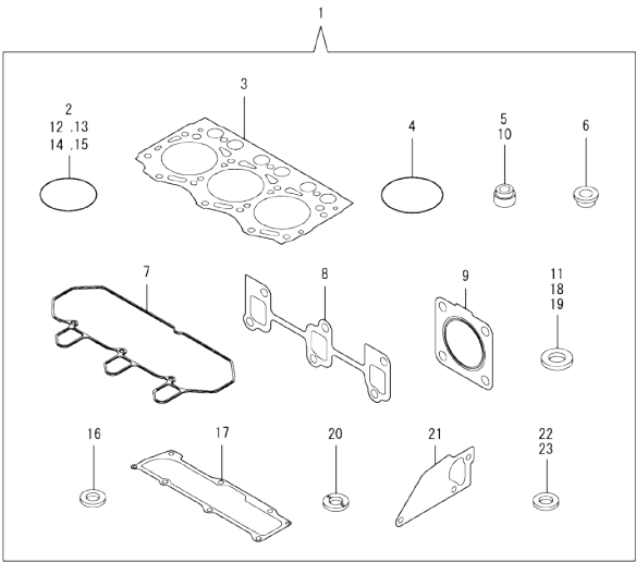
Fig.17. GASKET SET
