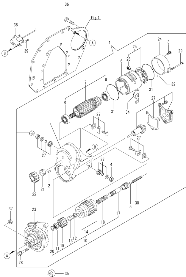
Fig.15. STARTER MOTOR
