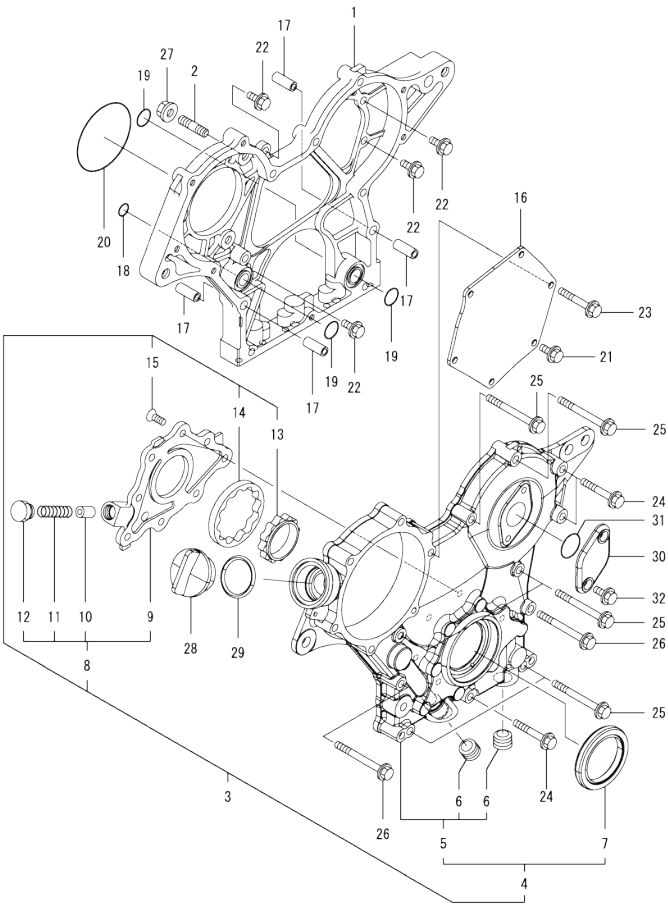
Fig.2. GEAR HOUSING
