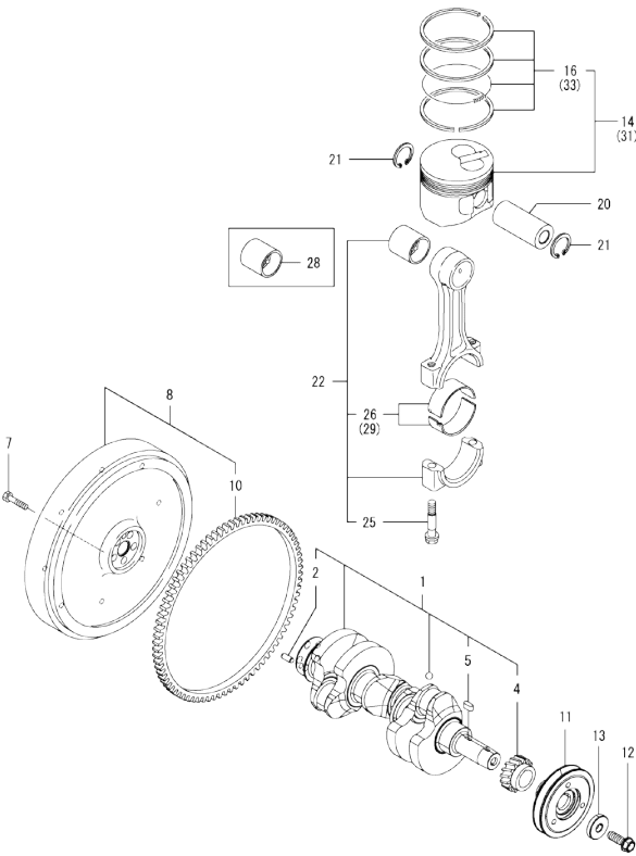
OCD50-M05870 ENGINE Fig.7. CRANKSHAFT & PISTON
