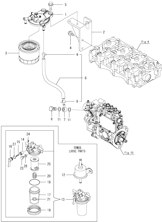
Fig.13. FUEL PIPE
