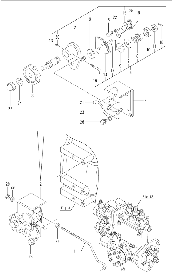
Fig.17. CONTROL EQUIPMENT
