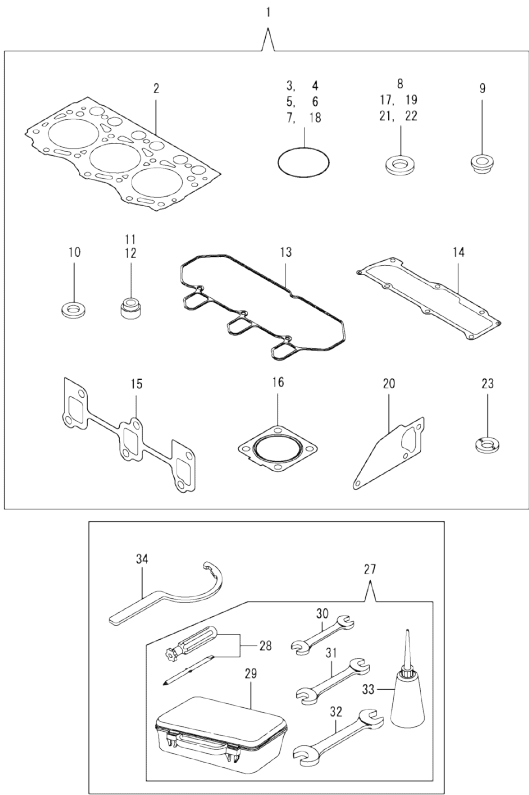
Fig.23. GASKET SET
