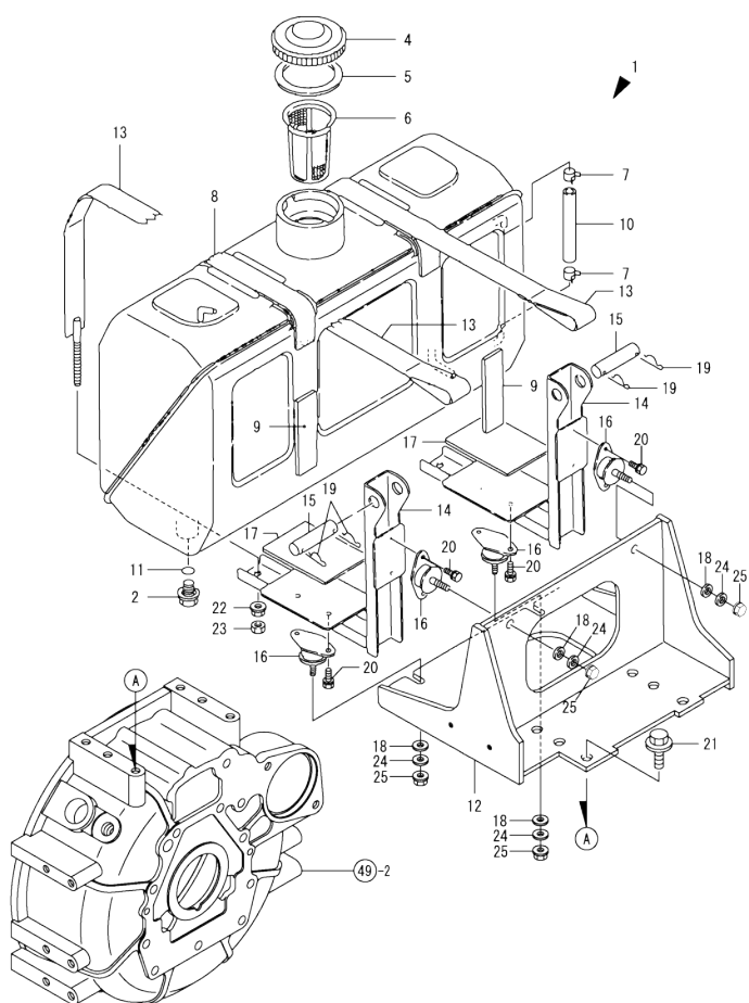
Fig.62. FUEL TANK
