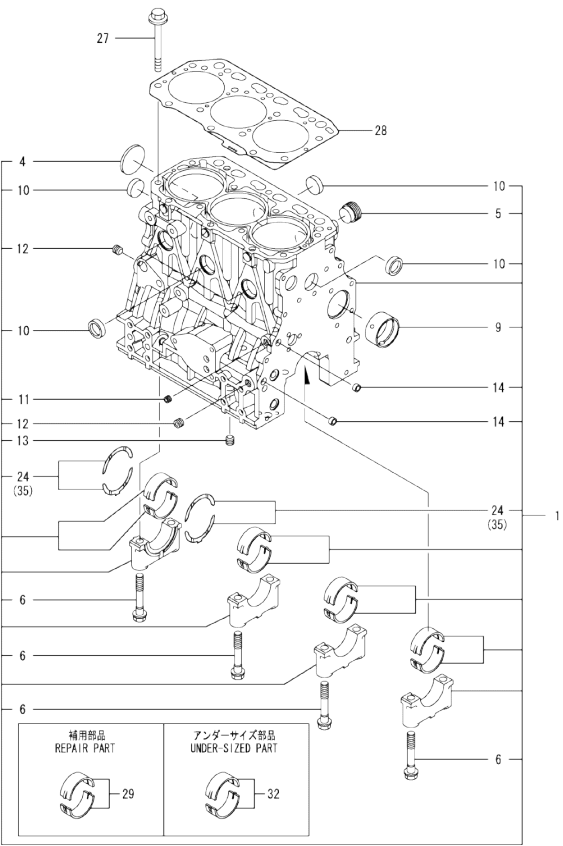
Fig.24. CYLINDER BLOCK
