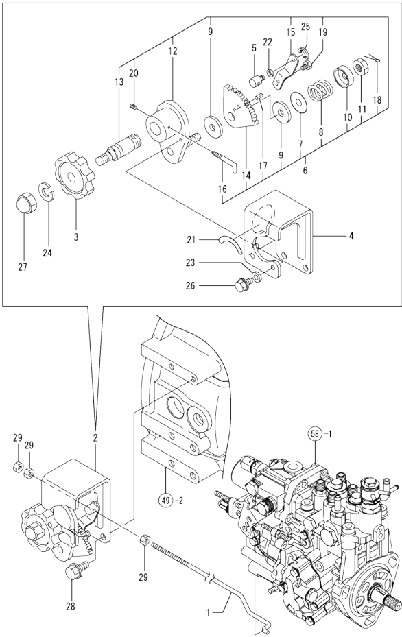
Fig.63. CONTROL DEVICE
