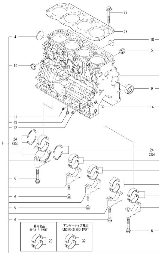
Fig.47. CYLINDER BLOCK
