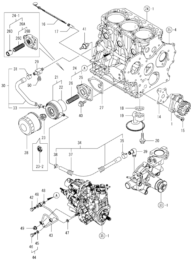
Fig.32. LUB. OIL SYSTEM
