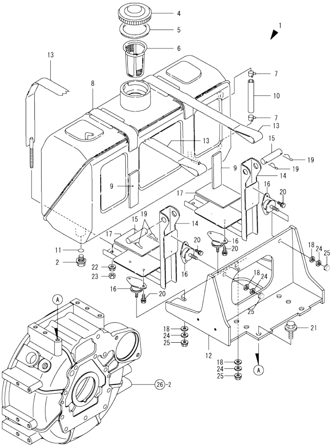
Fig.39. FUEL TANK
