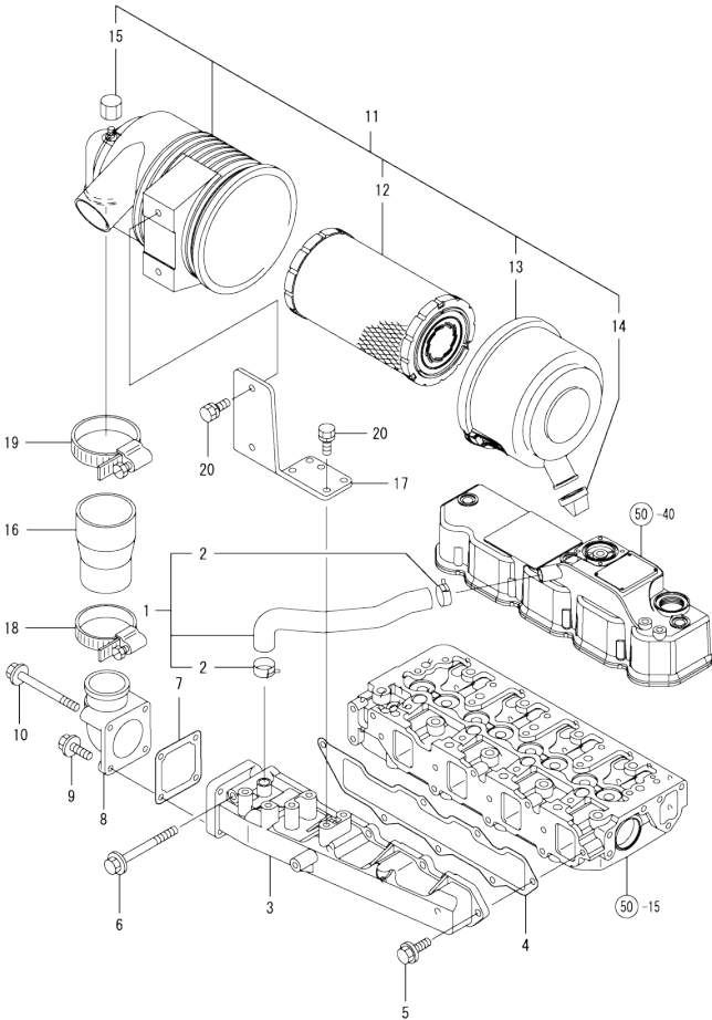
Fig.51. SUCTION MANIFOLD & AIR CLEANER
