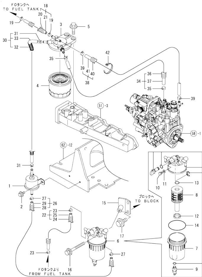
Fig.61. FUEL PIPE
