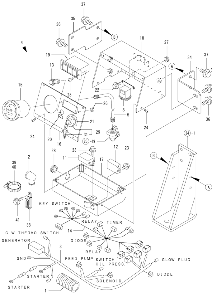
Fig.44. INSTRUMENT PANEL
