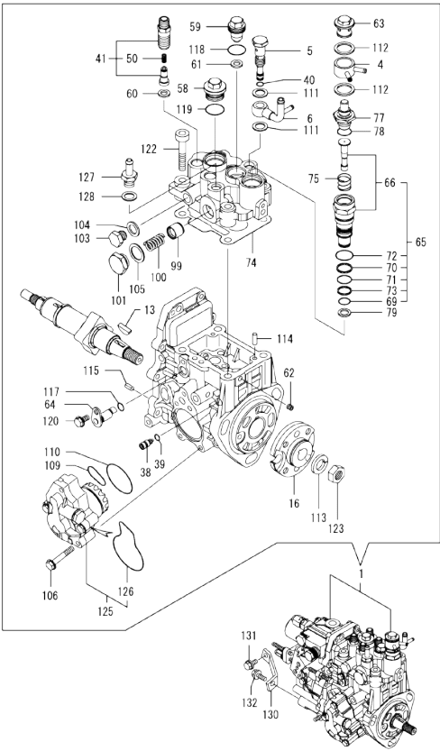
Fig.58. FUEL INJECTION PUMP
