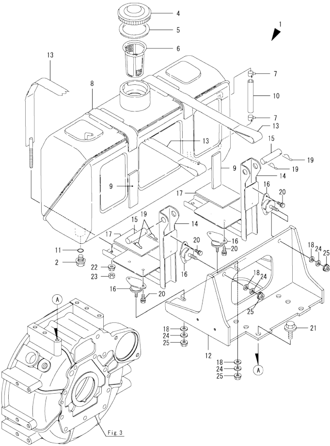
Fig.16. FUEL TANK
