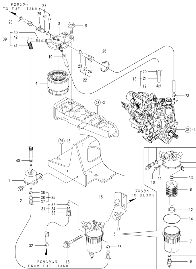
Fig.38. FUEL PIPE
