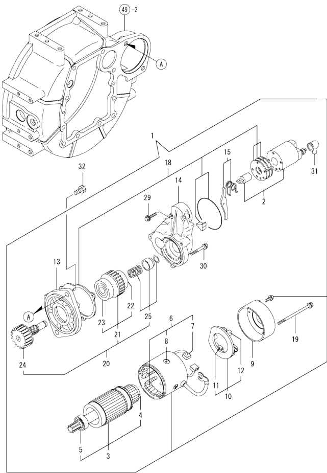
Fig.64. STARTER MOTOR
