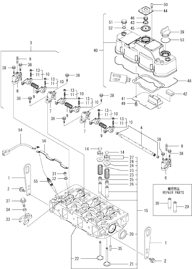
Fig.27. CYLINDER HEAD & BONNET
