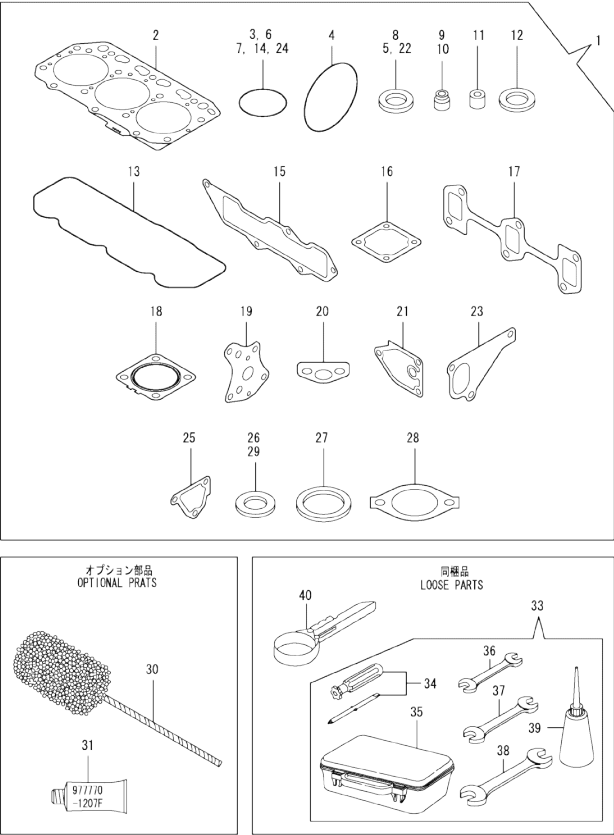
Fig.46. GASKET SET
