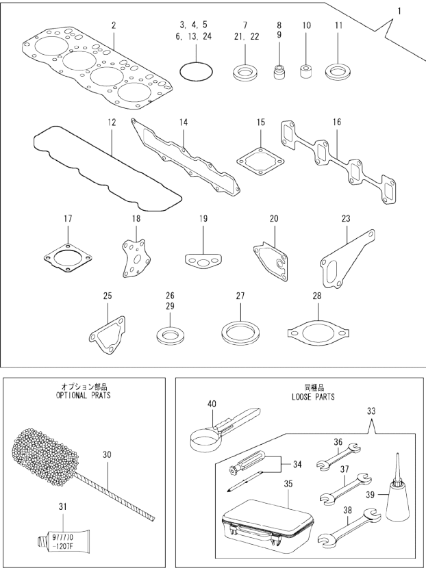
Fig.69. GASKET SET
