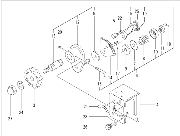
Fig.40. CONTROL DEVICE
