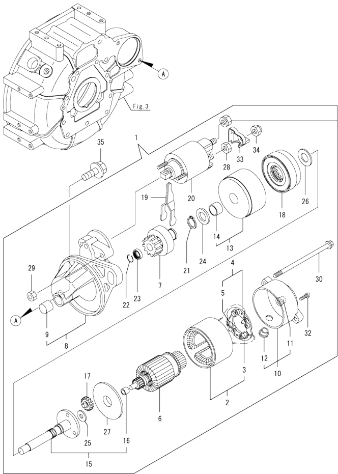
OCE10-M27001 YPU23V/YPU23V-1 Fig.18. STARTER MOTOR
