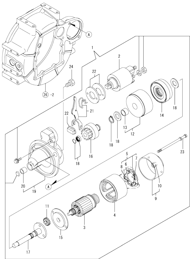
Fig.41. STARTER MOTOR
