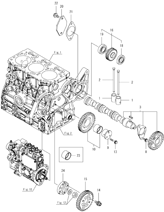
Fig.6. CAMSHAFT & DRIVING GEAR
