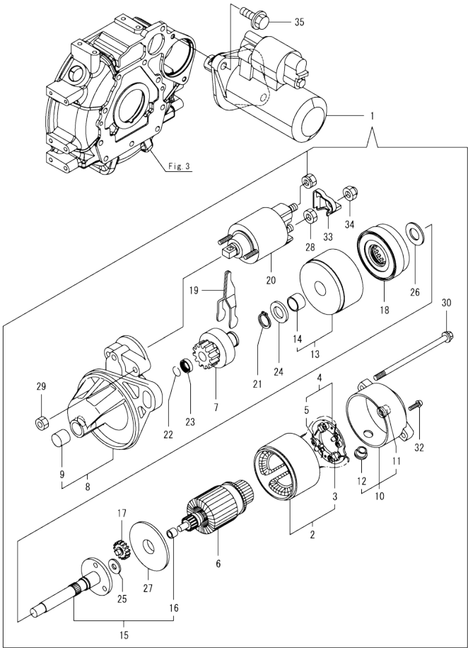
Fig.14. STARTER MOTOR
