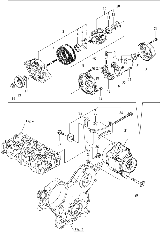
OCD50-M05250 ENGINE Fig.16. GENERATOR
