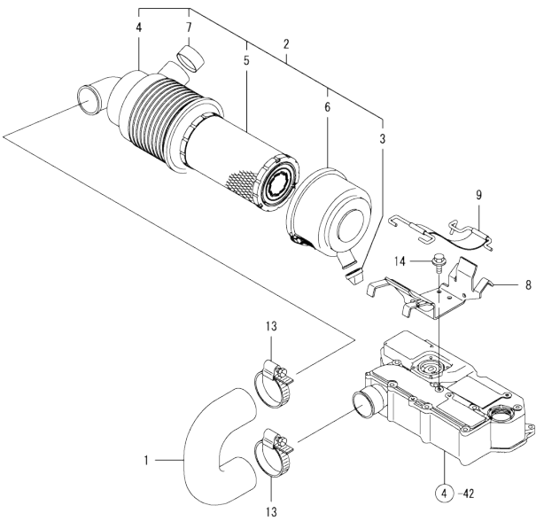
OCR10-M57400 ENGINE Fig.5. AIR CLEANER
