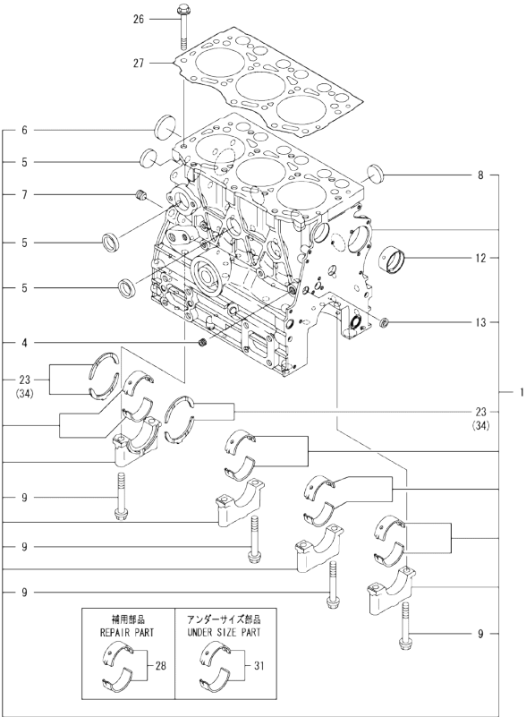
Fig.1. CYLINDER BLOCK
