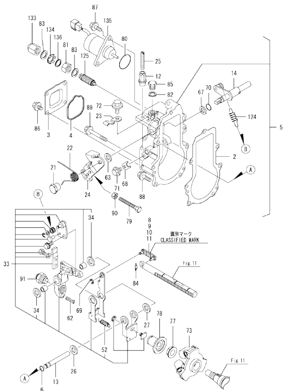
Fig.12. GOVERNOR
