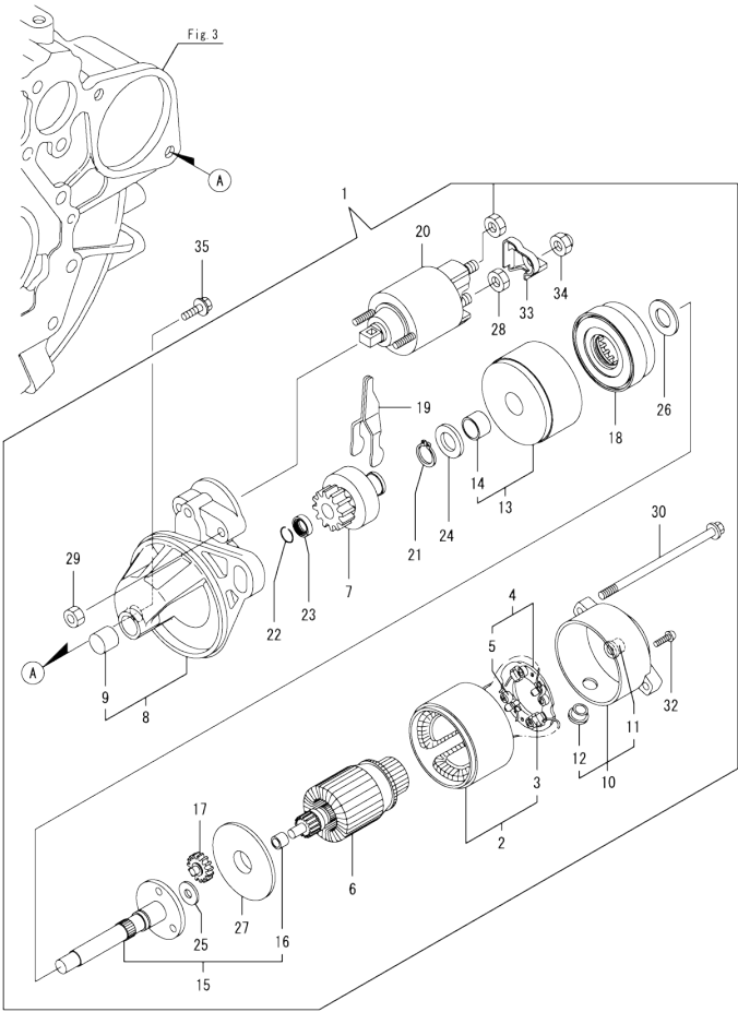
Fig.15. STARTING MOTOR
