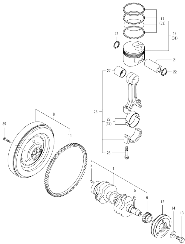
0CW10-M58500 ENGINE SECTION Fig.7. CRANKSHAFT & PISTON
