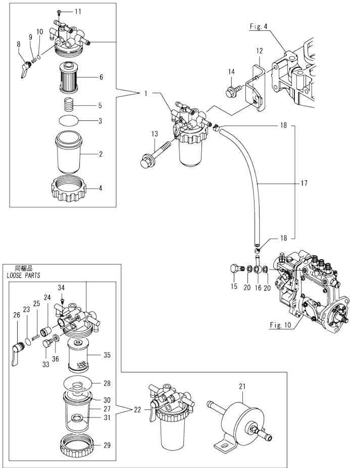
Fig.13. FUEL LINE
