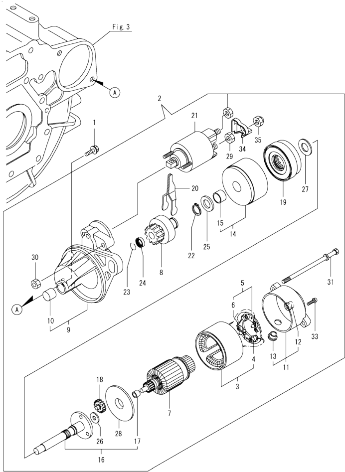
0CW10-M58500 ENGINE SECTION Fig.14. STARTING MOTOR
