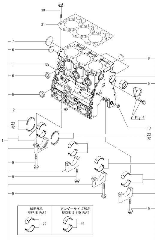
0CW10-M58500 ENGINE SECTION Fig.1. CYLINDER BLOCK
