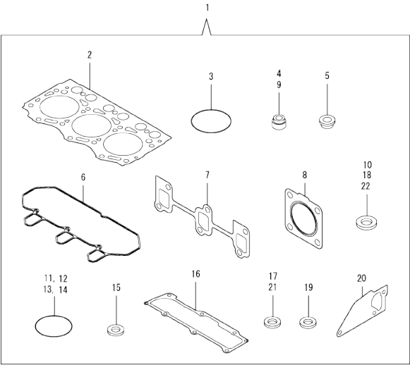
Fig.17. GASKET SET
