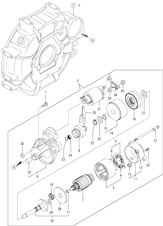
Fig.14. STARTING MOTOR
