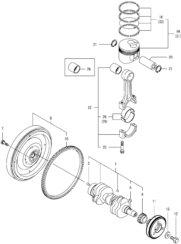
OCD50-M04490 ENGINE Fig.7. CRANKSHAFT & PISTON
