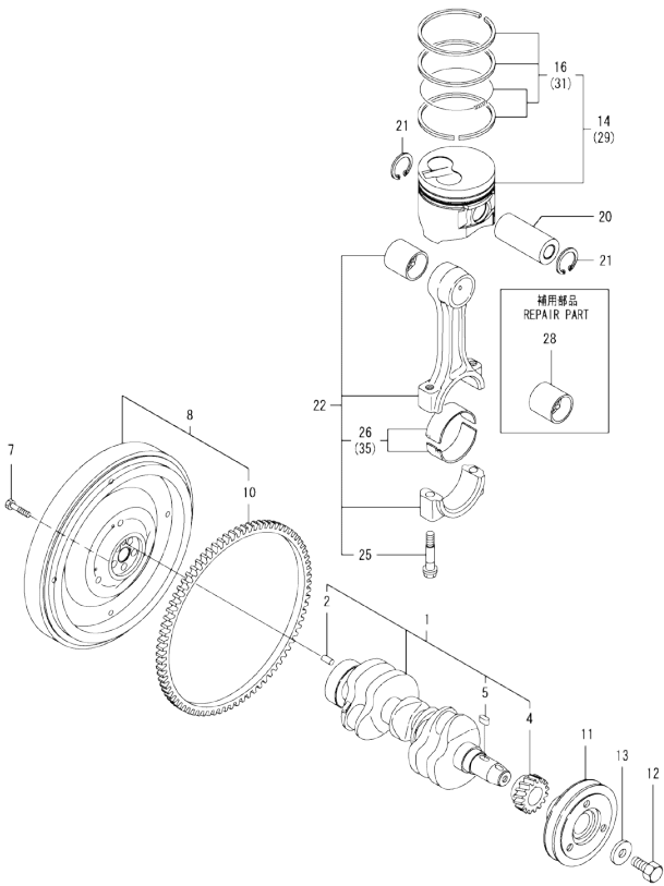
Fig.8. CRANKSHAFT & PISTON
