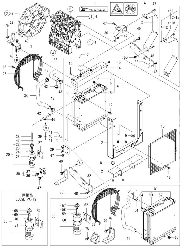
0CW10-M39500 ENGINE Fig.11. RADIATOR
