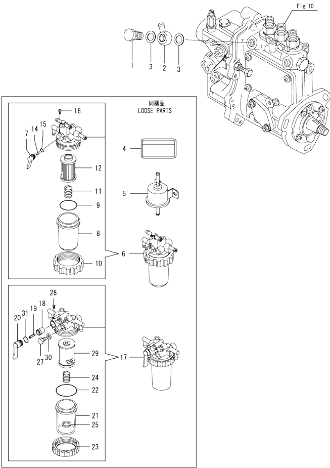
Fig.13. FUEL FILTER
