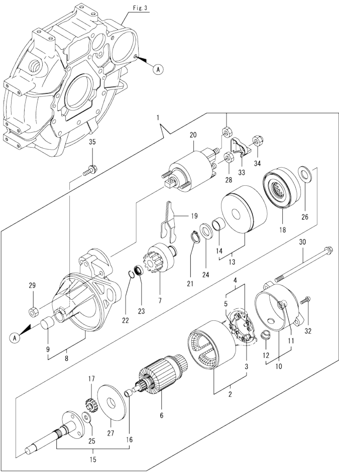
0CW10-M67100 3TNV76-PAMM Fig.14. STARTING MOTOR
