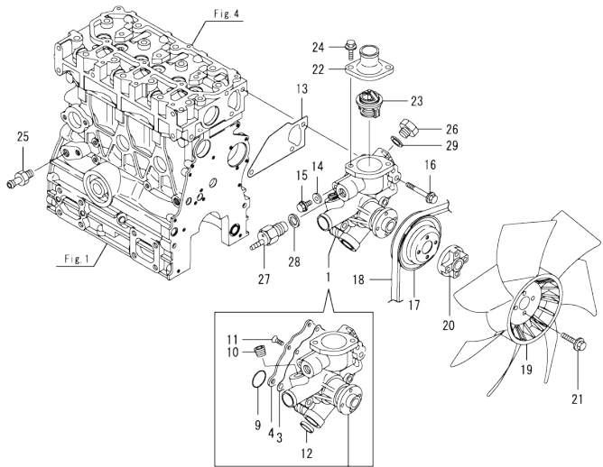
Fig.9. COOLING WATER SYSTEM
