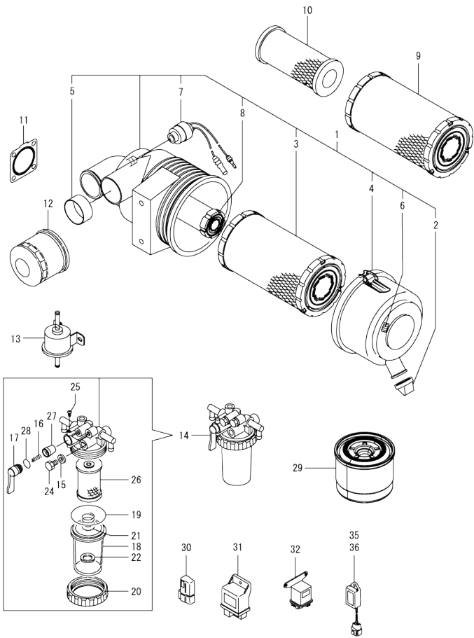
Fig.16. ACCESSORY
