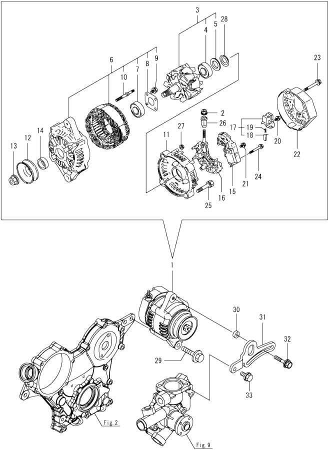
OCD50-M04300 ENGINE Fig.15. GENERATOR
