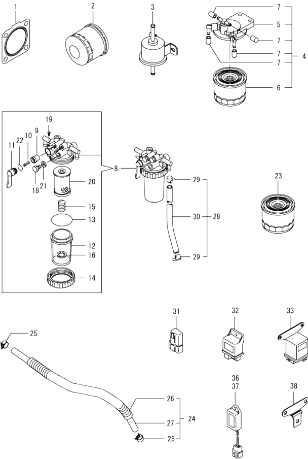
Fig.16. ACCESSORY
