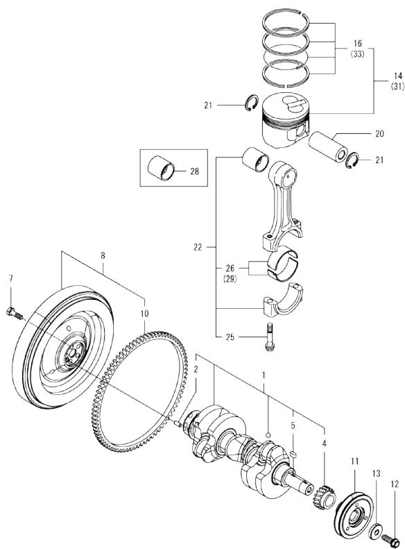
Fig.7. CRANKSHAFT & PISTON
