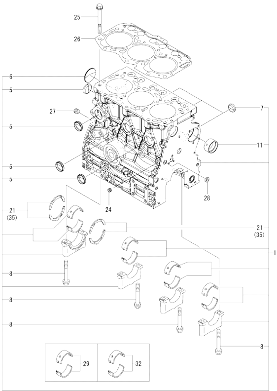
Fig.1. CYLINDER BLOCK
