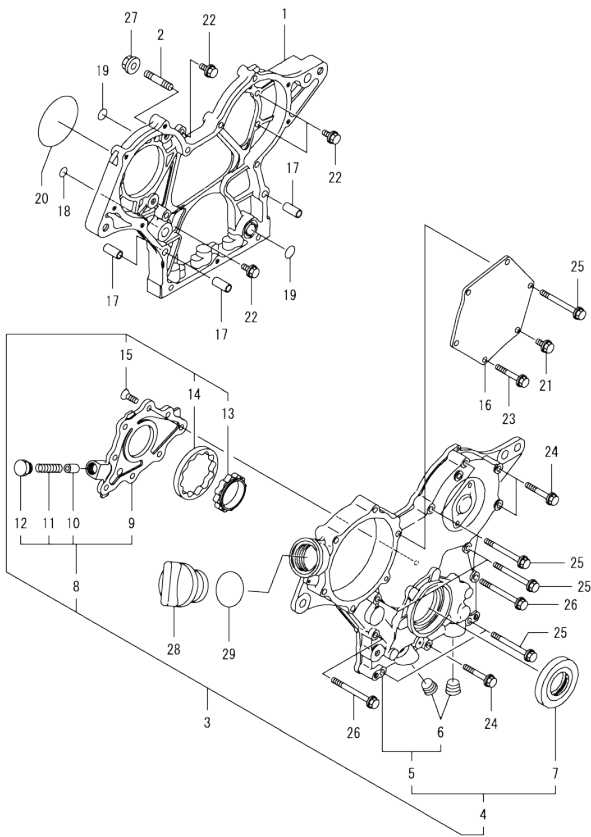
Fig.2. GEAR HOUSING
